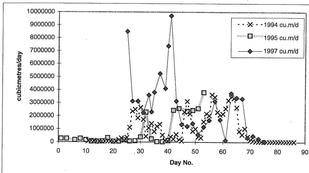
Figure 5. Water discharge (cubic metres) in Eastern River in 1994, 1995, and 1997. Day 1 is 29 May.
