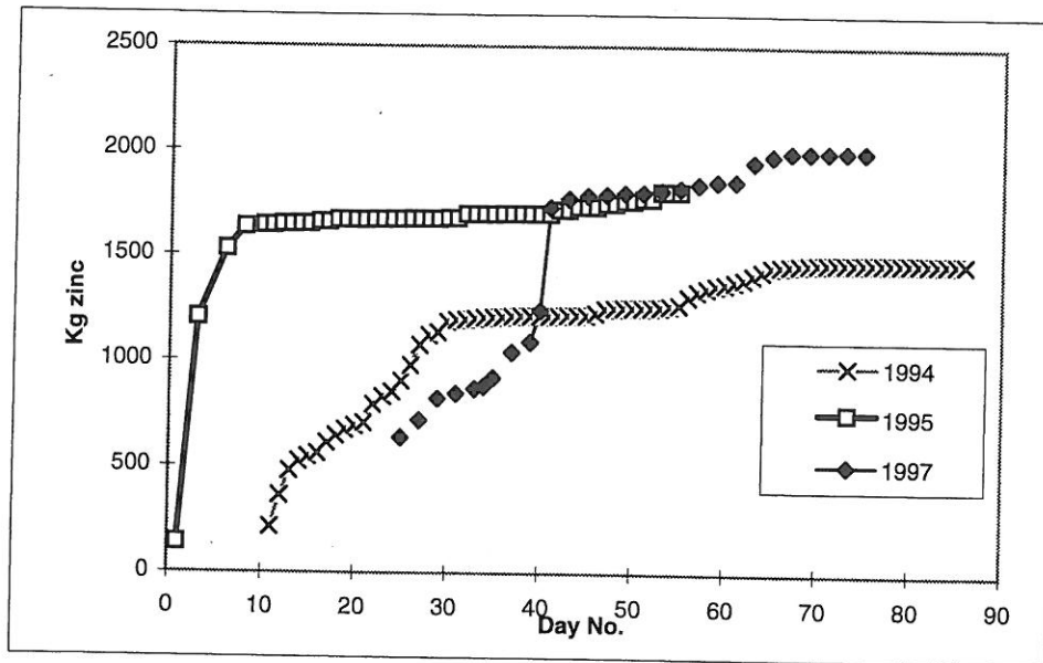
Figure 4. Accumulated zinc (kg) transported out through Eastern River in 1994, 1995, and 1997. Day 1 is 29 May.
