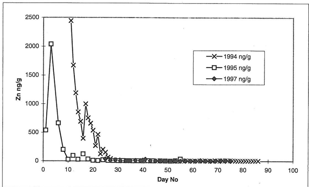
Figure 3. Zinc concentrations in Eastern River at station V1 in 1994, 1995, and 1997. Day 1 is 29 May.
