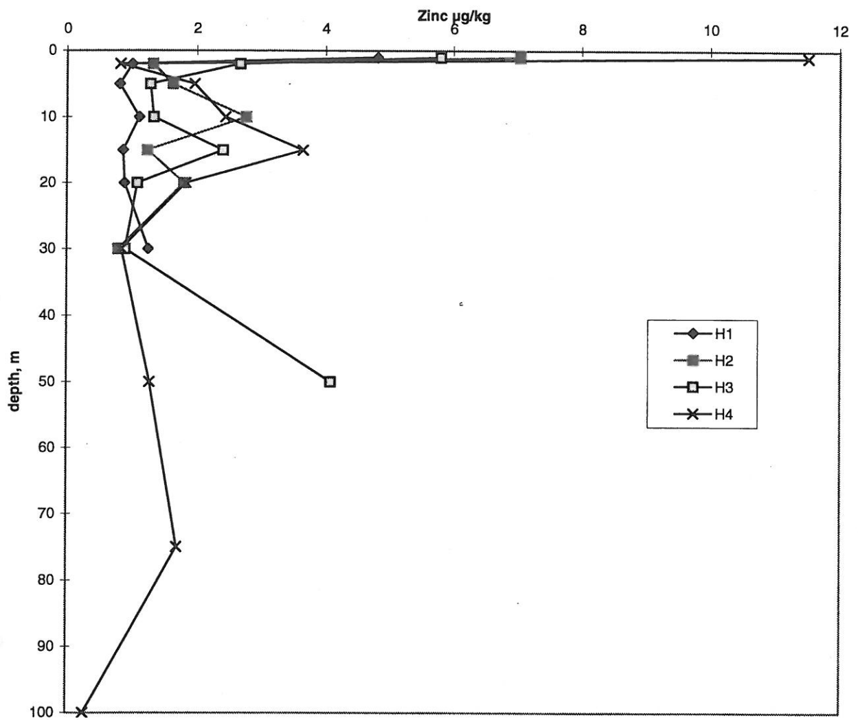
Figure 2. Zinc concentrations ( \mu\text{g}/\text{kg} ) at four sea water column stations (H1-4).
