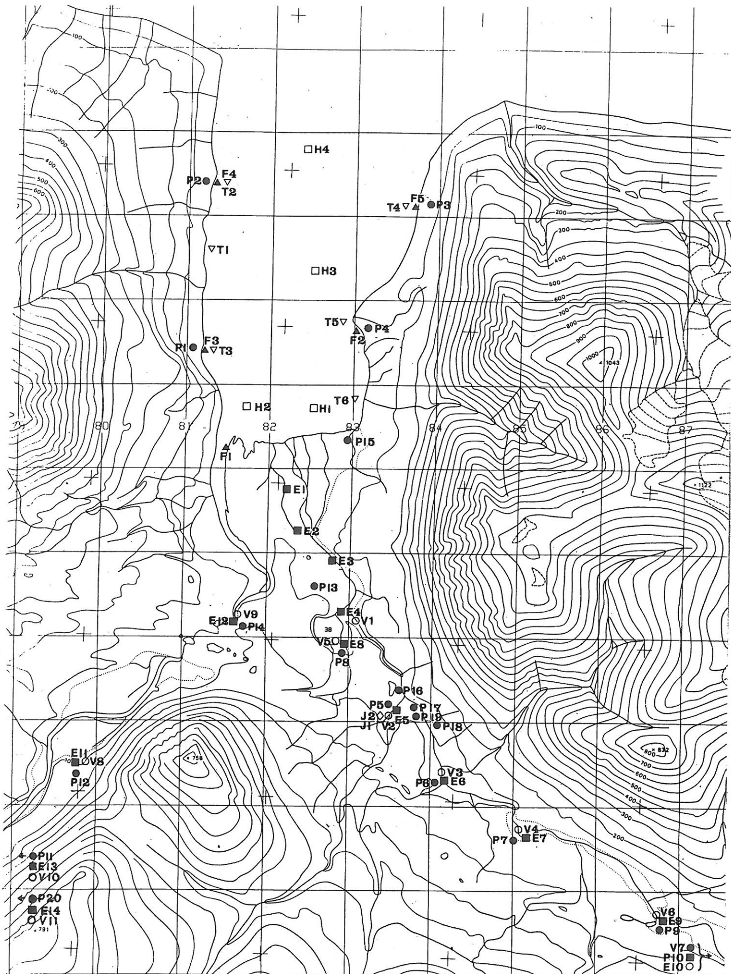
Figure 1. Stations in Citronen Fjord: Fish (▲ F), Seaweed (▽ T), Sea water column (□ H), River sediment (■ E), Soil (◇ J); Plant and faeces (● P) and Fresh water (○ V). Soil was sampled only in 1994.
