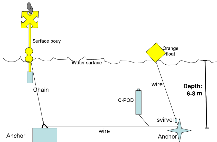
Figure 2.2.2. The deployment system used for mooring C-PODs. The set-up has been designed so that the instruments can be lifted to the surface by hand by pulling in the orange float (yellow square).
