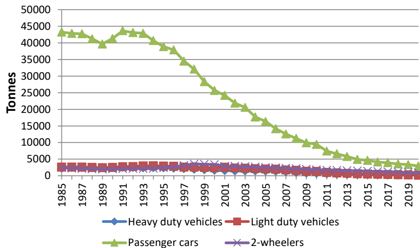
Figure 6.24 NMVOC emissions (tonnes) per vehicle type for road transport 1985-2020.
