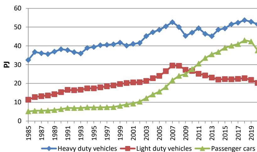
Figure 6.6 Diesel fuel consumption per vehicle type for road transport 1985-2020.
