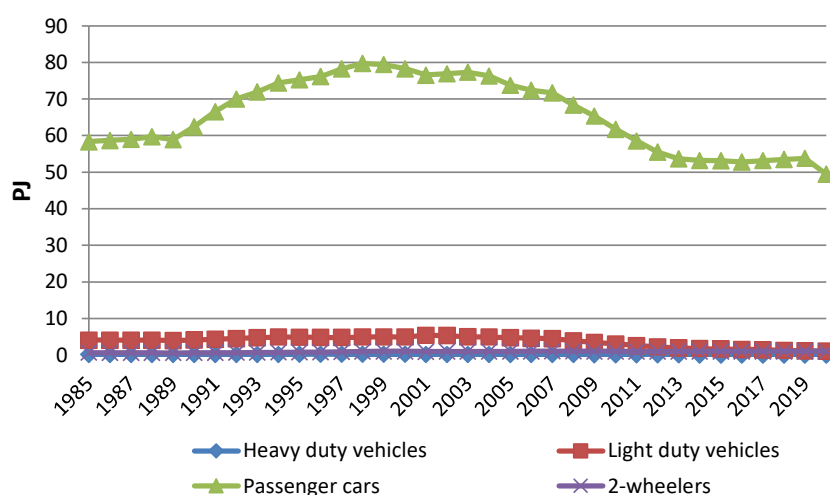
Figure 6.5 Gasoline fuel consumption per vehicle type for road transport 1985-2020.
