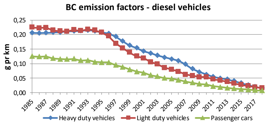
Figure 4.11 Fuel and km related BC emission factors per vehicle type for Danish road transport (1985-2020).
