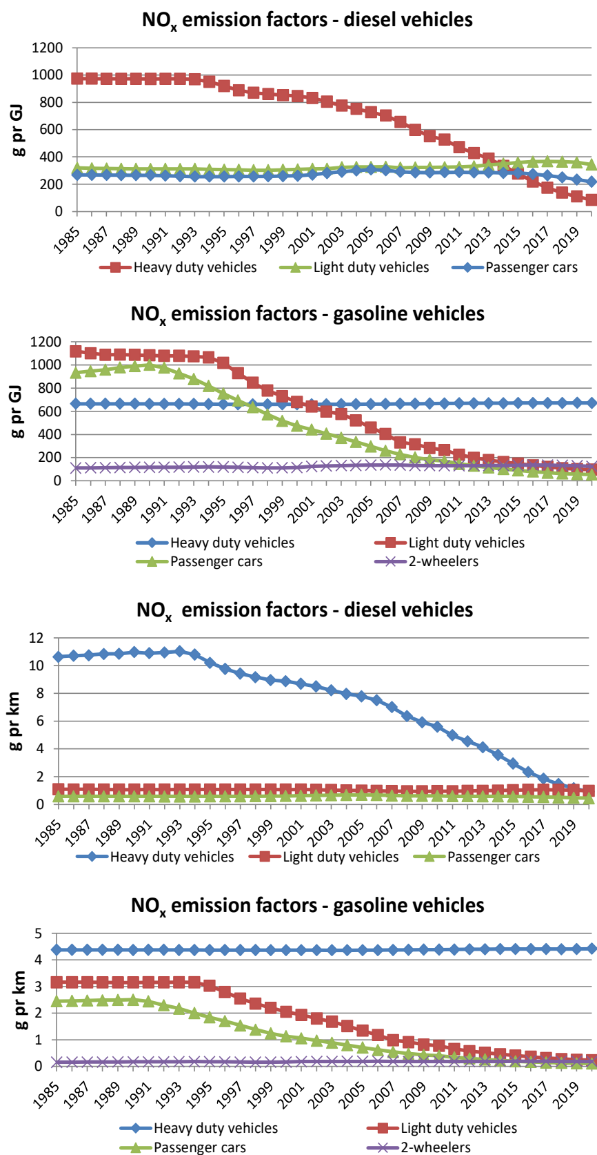
Figure 4.7 Fuel and km related NO x emission factors per vehicle type for Danish road transport (1985-2020).
