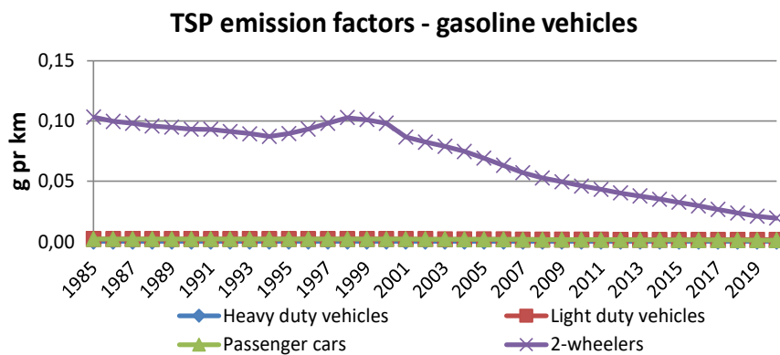
Figure 4.10 Fuel and km related TSP emission factors per vehicle type for Danish road transport (1985-2020).
