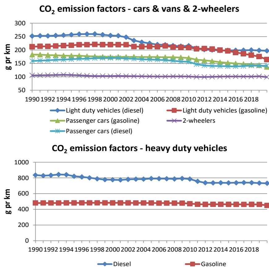
Figure 4.6 Km related CO 2 emission factors per vehicle type for Danish road transport (1990-2020).
