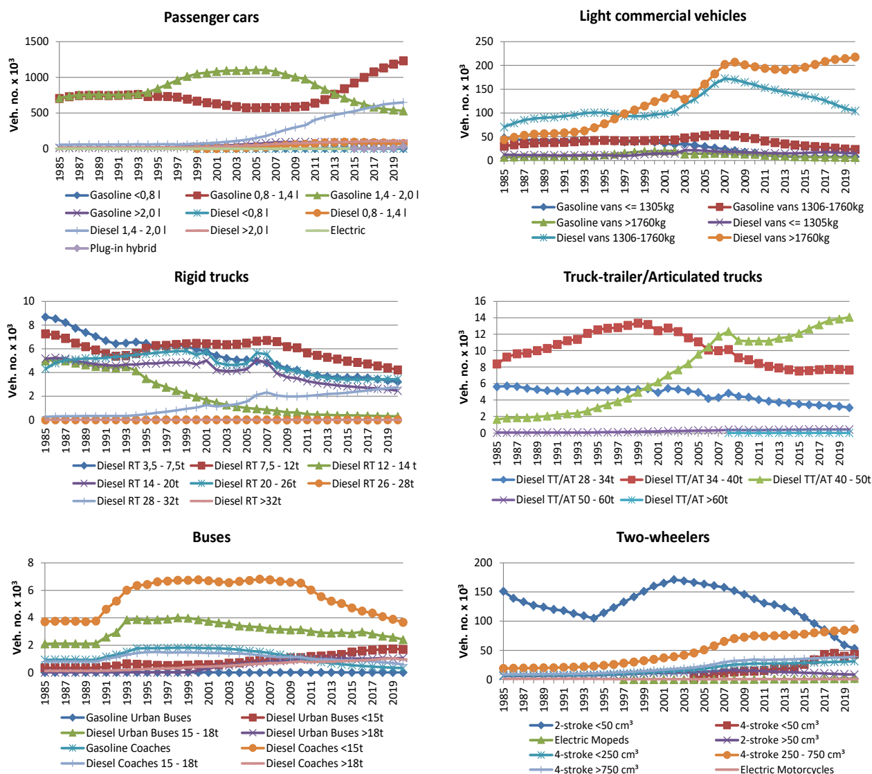
Figure 4.1 Number of vehicles in sub-classes in 1985-2020.
