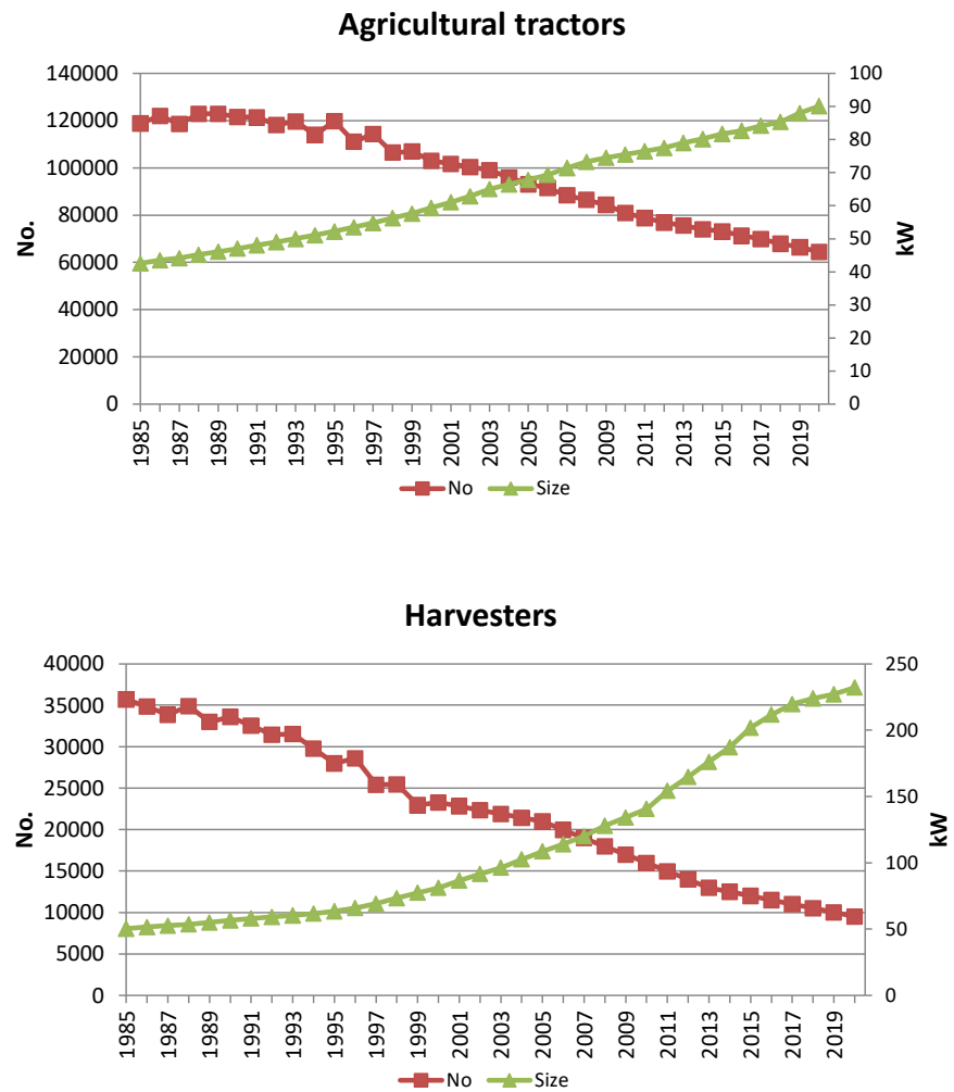
Figure 5.5 Total numbers and average engine size for tractors and harvesters from 1985 to 2020.
