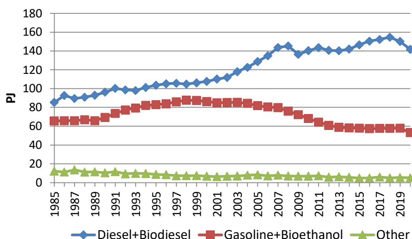
Figure 6.1 Fuel consumption per fuel type for domestic transport 1985-2020.
