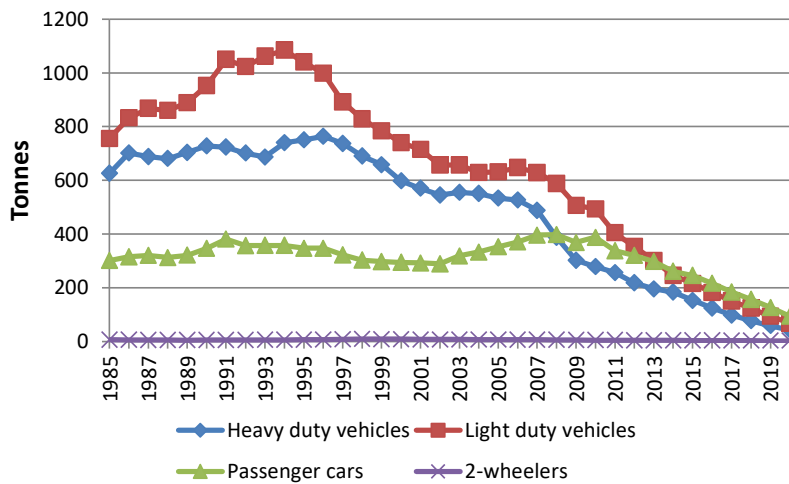
Figure 6.27 BC emissions (tonnes) per vehicle type for road transport 1985-2020.
