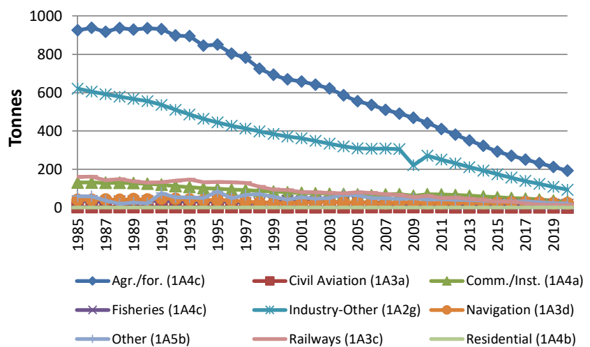
Figure 6.36 BC emissions (tonnes) in NFR sectors for other mobile sources 1985-2020.
