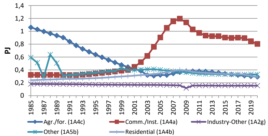
Figure 6.10 Gasoline fuel consumption in CRF sectors for other mobile source 1985-2020.
