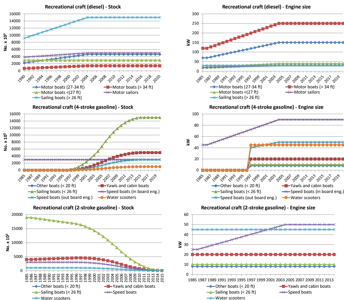
Figure 5.11 Stock and engine size development for recreational craft 1985-2020.
