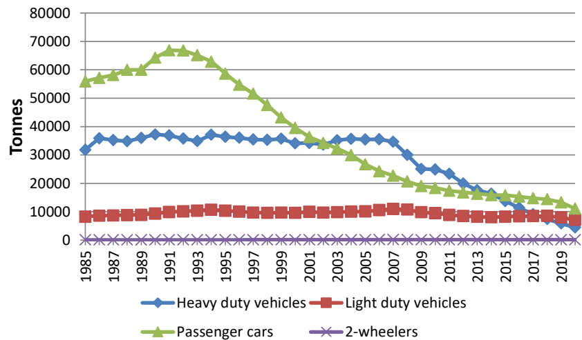
Figure 6.23 \text{NO}_x emissions (tonnes) per vehicle type for road transport 1985-2020.
