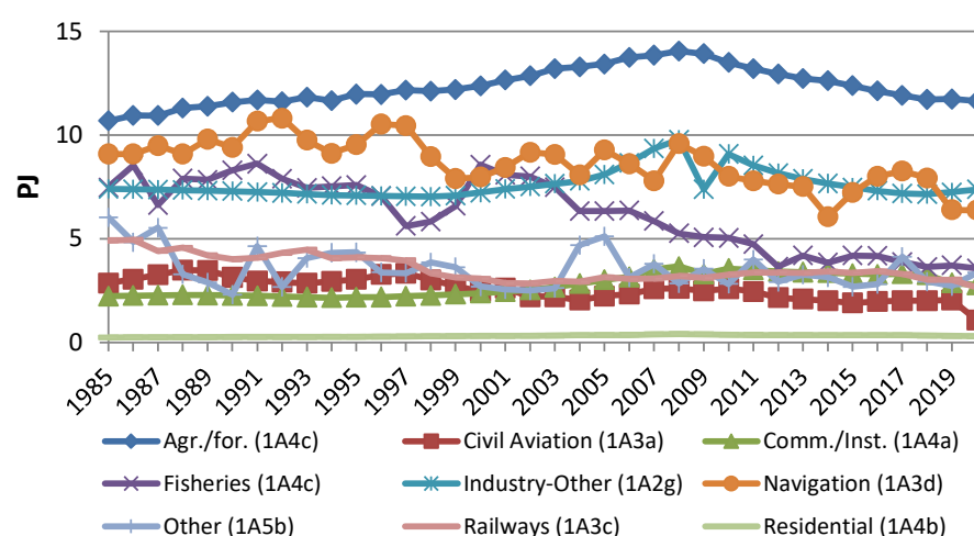
Figure 6.8 Total fuel consumption in CRF sectors for other mobile sources 1985-2020.
