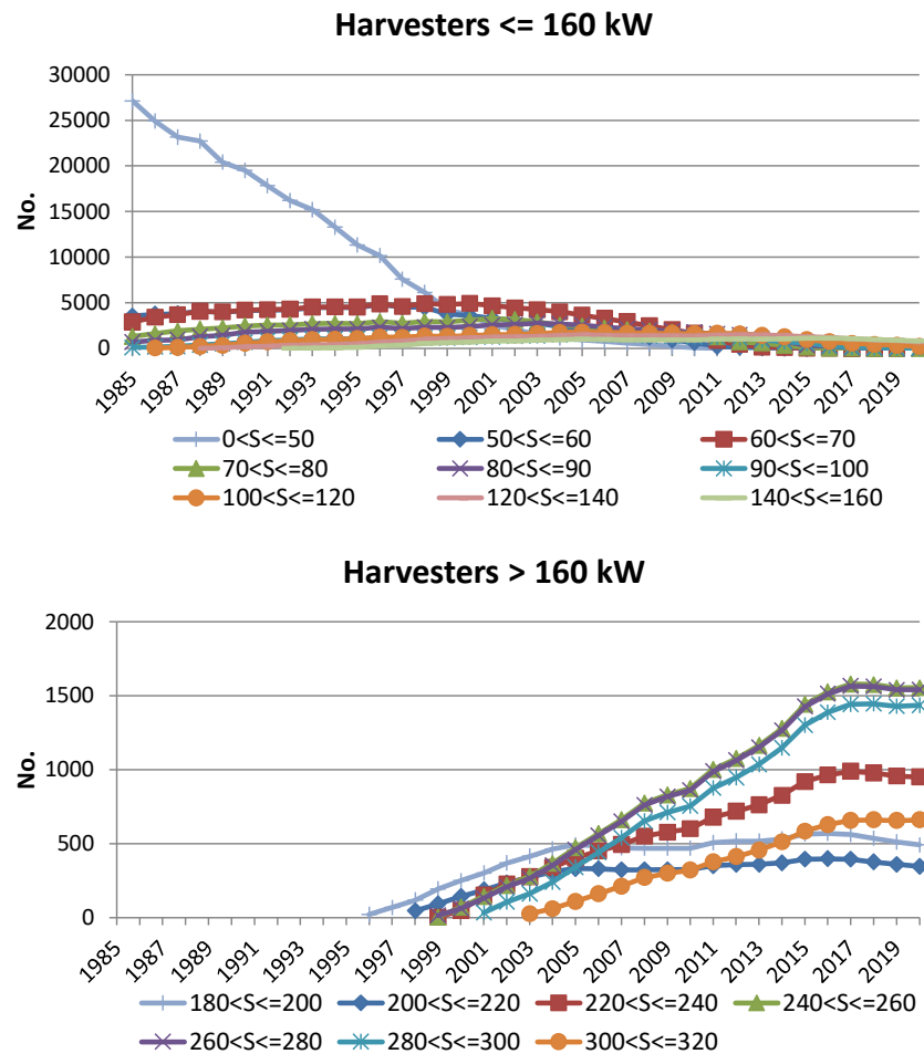
Figure 5.4 Total numbers in kW classes for harvesters from 1985 to 2020.
