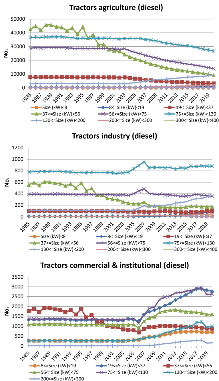
Figure 5.3 Total numbers in kW classes for tractors used in Agriculture, Industry and Commercial/Institutional from 1985 to 2020.
