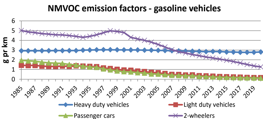
Figure 4.8 Fuel and km related NMVOC emission factors per vehicle type for Danish road transport (1985-2020).
