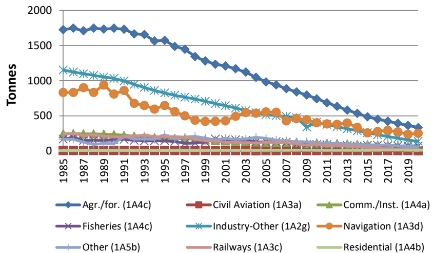
Figure 6.35 TSP emissions (tonnes) in NFR sectors for other mobile sources 1985-2020.
