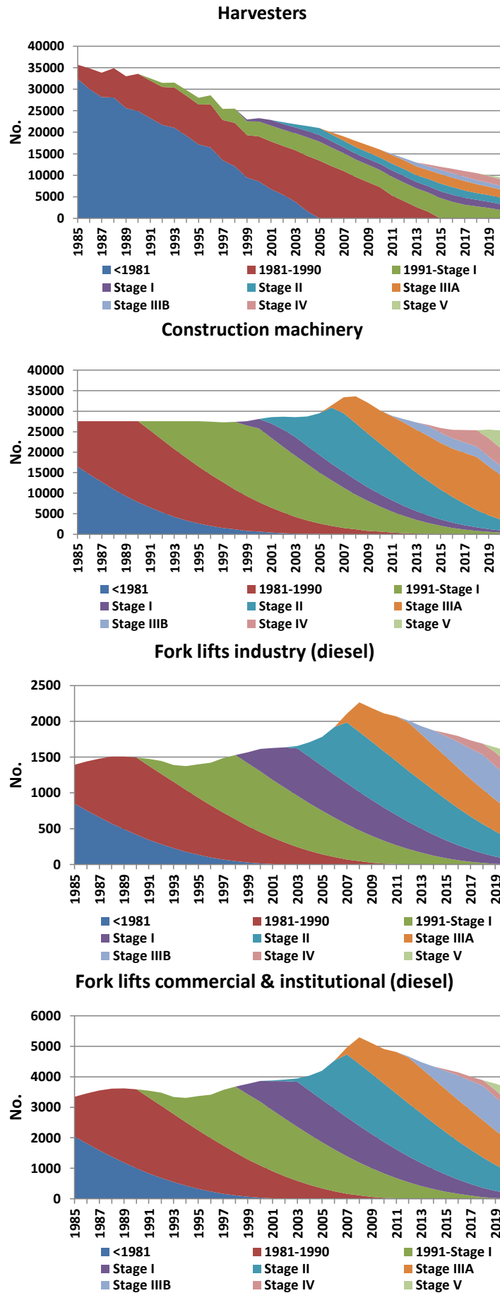
Figure 5.8 Layer distribution for tractors, harvesters, construction machinery and diesel fork lifts (1985 to 2020).
