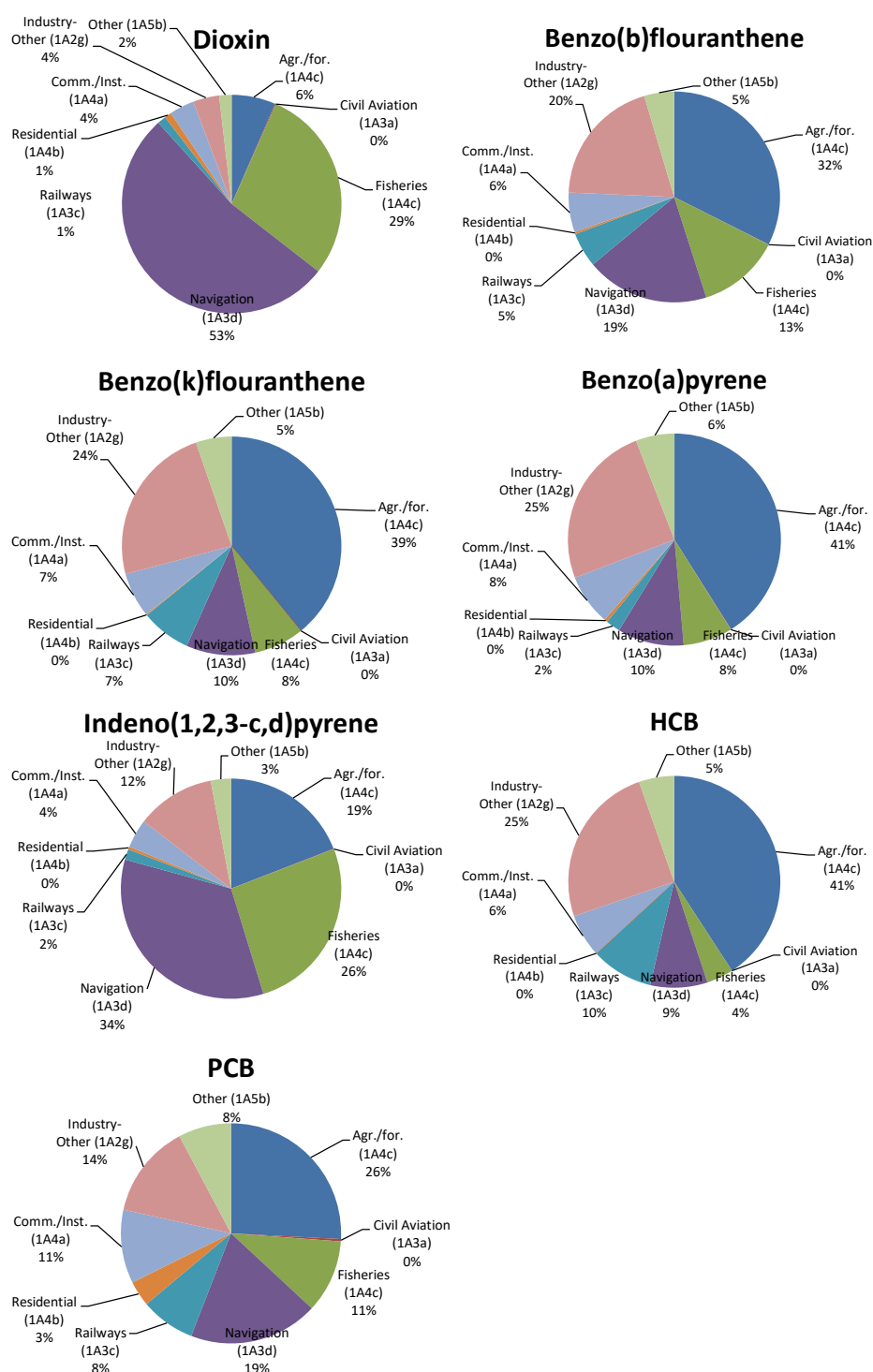
Figure 6.44 Dioxin, PAH, HCB and PCB emission shares for other mobile sources in 2020.
