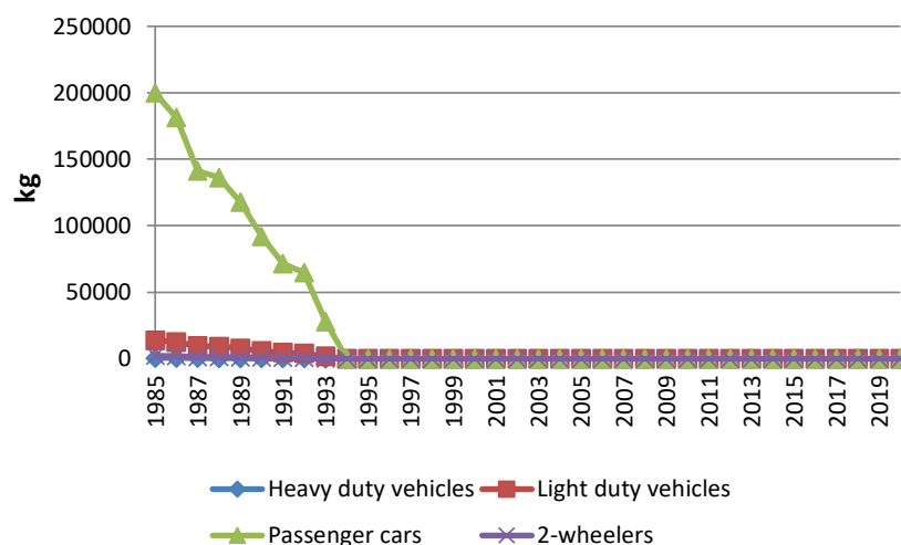
Figure 6.41 Pb emissions (kg) per vehicle type for road transport 1985-2020.
