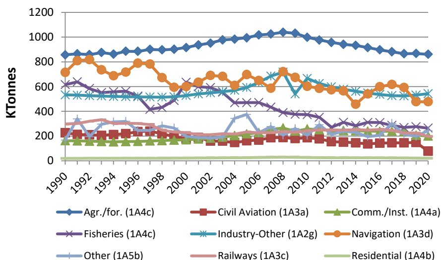
Figure 6.18 CO 2 emissions (ktonnes) in CRF sectors for other mobile sources 1990-2020.
