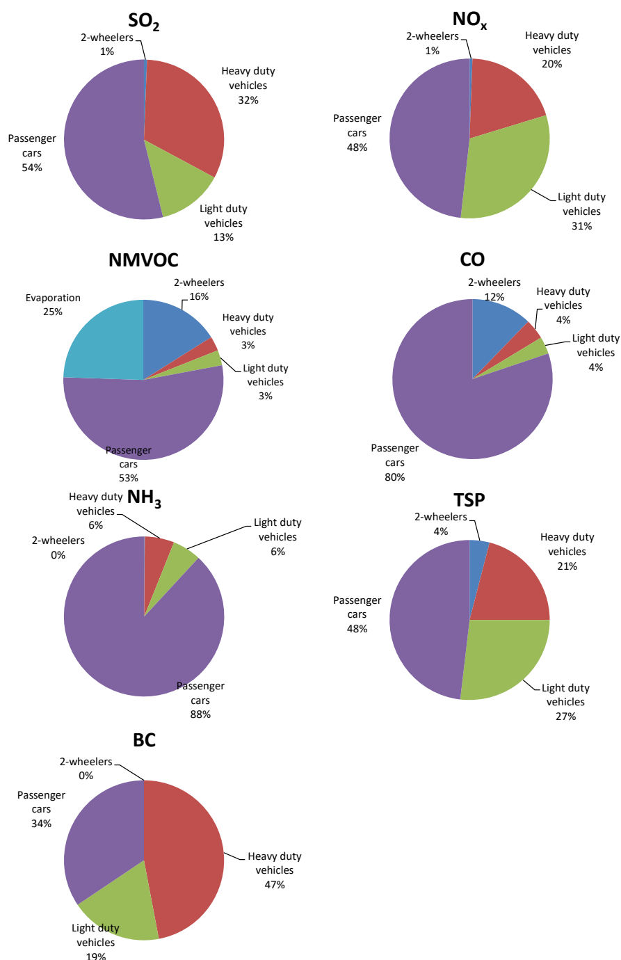
Figure 6.29 SO 2 , NO x , NMVOC, CO, NH 3 , PM and BC emission shares per vehicle type for road transport in 2020.
