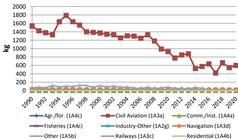
Figure 6.42 Pb emissions (kg) in NFR sectors for other mobile sources 1990-2020.
