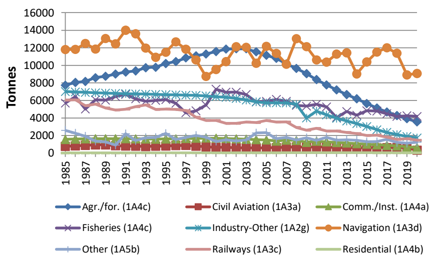
Figure 6.32 NO x emissions (tonnes) in NFR sectors for other mobile sources 1985-2020.
