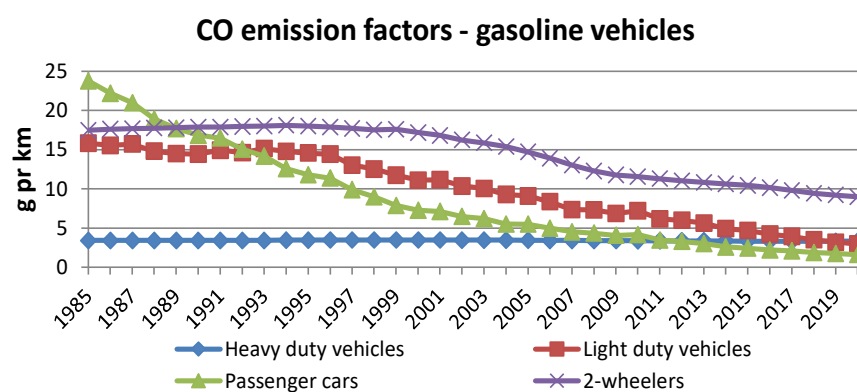
Figure 4.9 Fuel and km related CO emission factors per vehicle type for Danish road transport (1985-2020).
