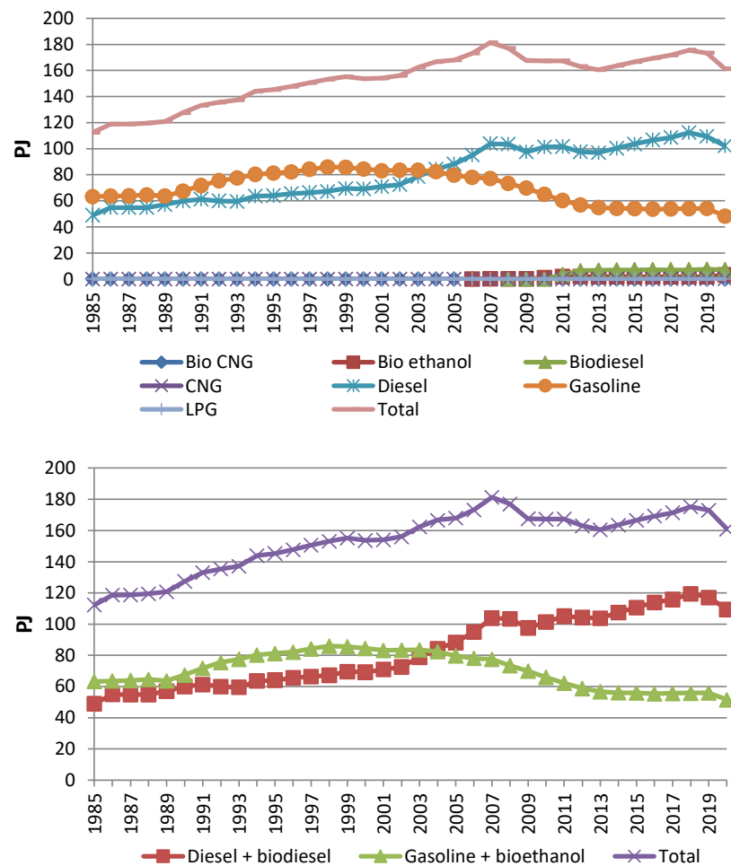
Figure 6.3 Fuel consumption per fuel type and as totals for road transport 1985-2020.
