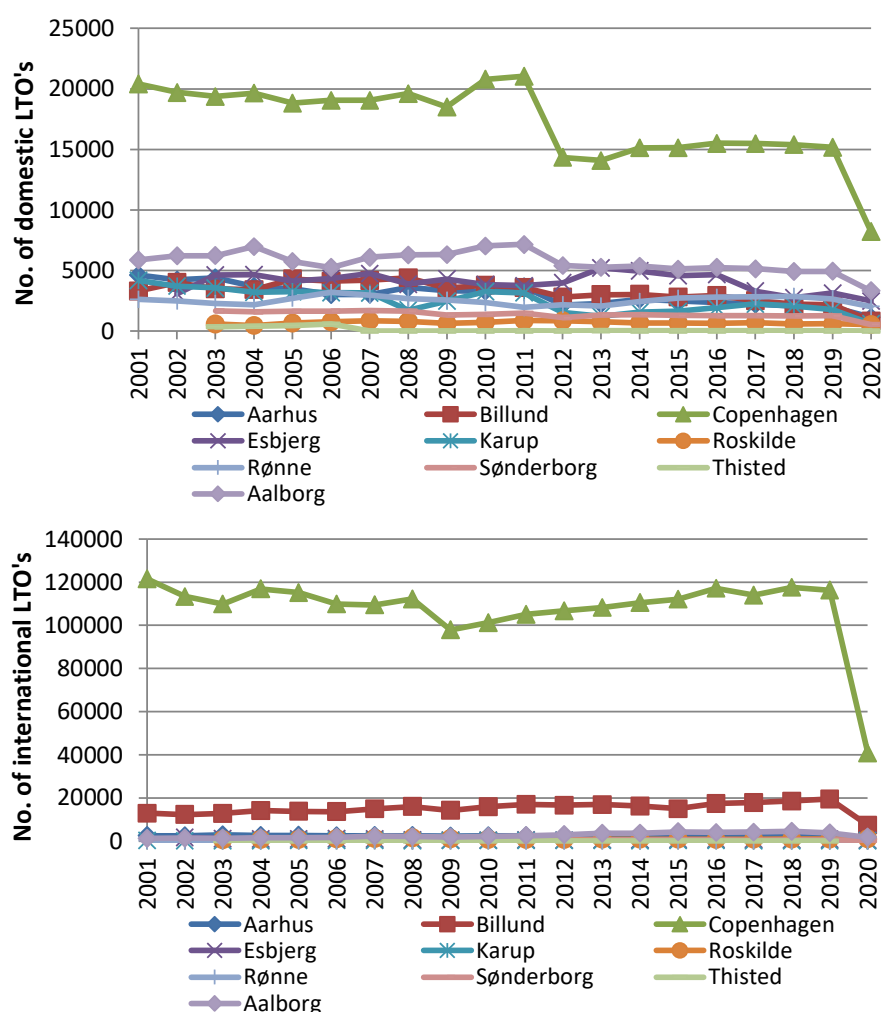
Figure 5.2 No. of LTO's for the most important airports in Denmark 2001-2020.
