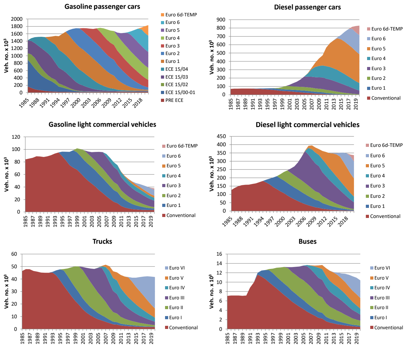
Figure 4.2 Layer distribution of vehicle numbers per vehicle type in 1985-2020.
