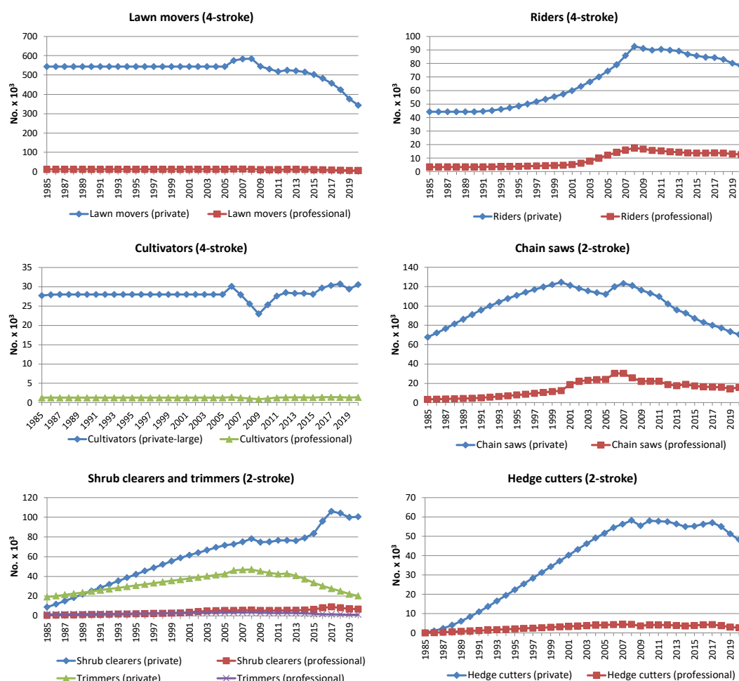
Figure 5.9 Stock developments 1985-2020 for the most important household and gardening machinery types.
