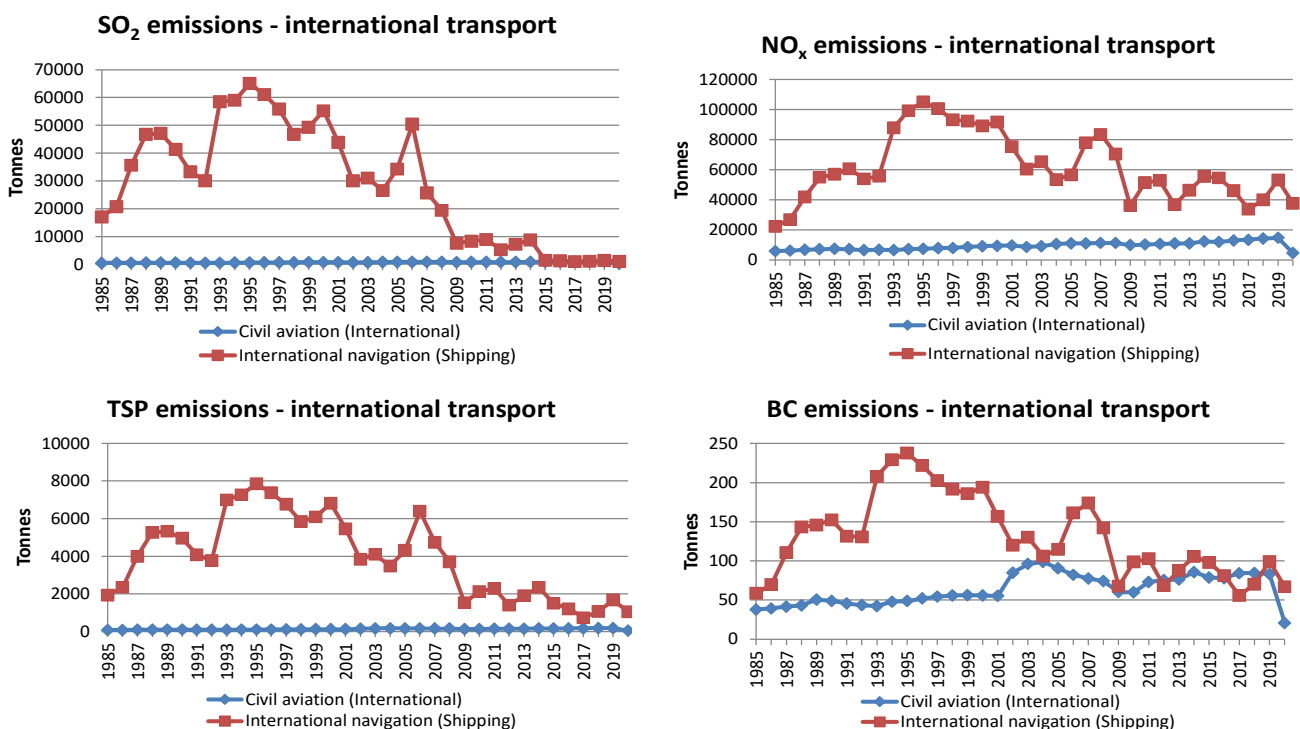
Figure 6.46 SO 2 , NO x , TSP and BC emissions for international transport 1985-2020.
