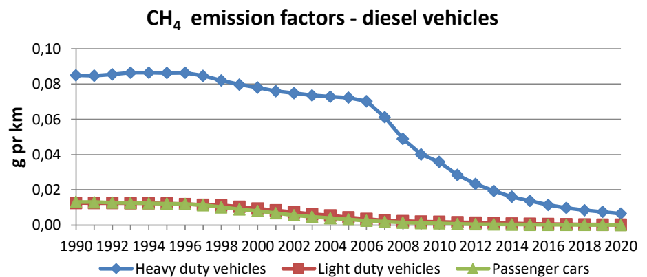
Figure 4.12 Fuel and km related CH 4 emission factors per vehicle type for Danish road transport (1990-2020).
