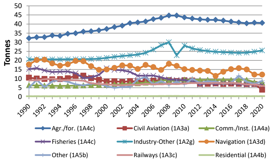
Figure 6.20 N 2 O emissions (tonnes) in CRF sectors for other mobile sources 1990-2020.
