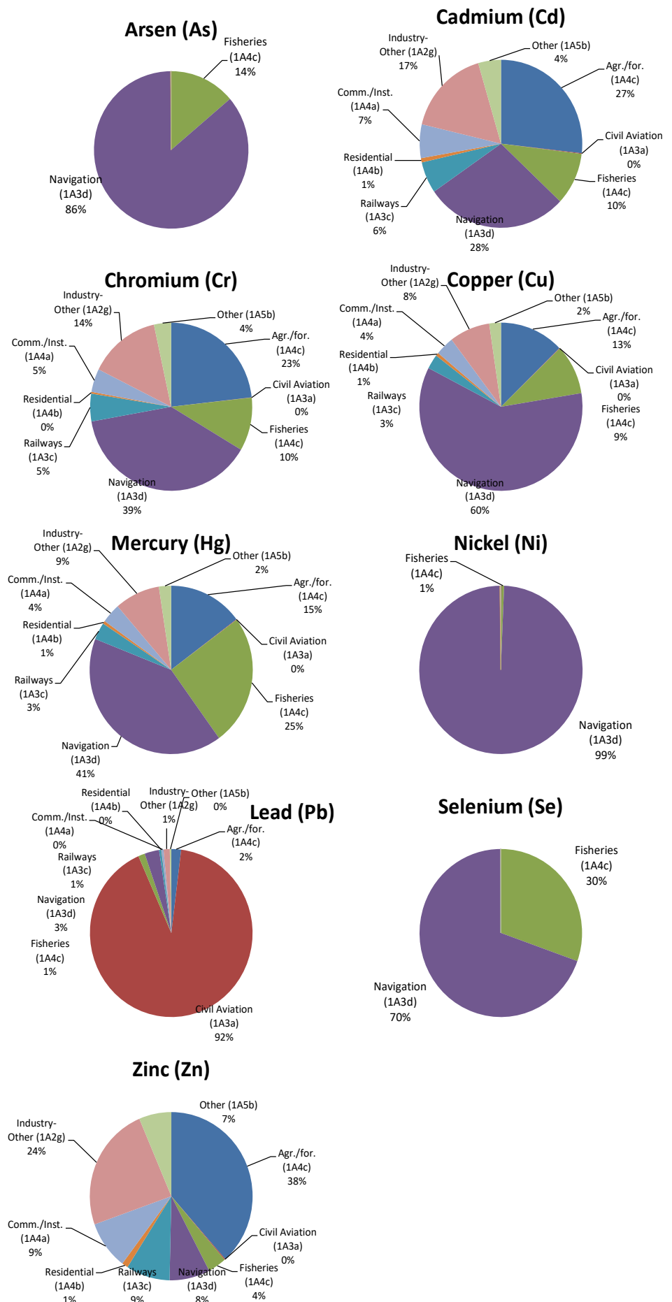
Figure 6.40 Heavy metal emission shares for other mobile sources in 2020.
