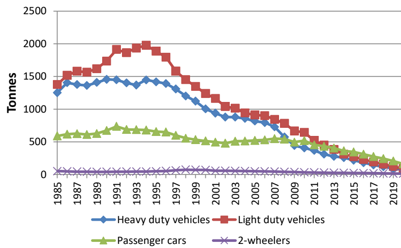
Figure 6.26 PM emissions (tonnes) per vehicle type for road transport 1985-2020.
