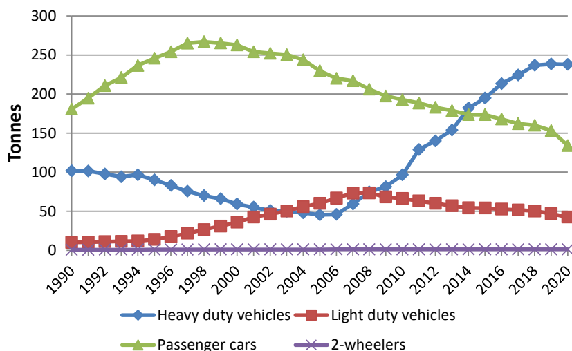
Figure 6.16 N 2 O emissions (tonnes) per vehicle type for road transport 1990-2020.
