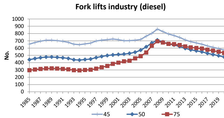
Figure 5.6 1985-2020 stock development for specific types of construction machinery.
