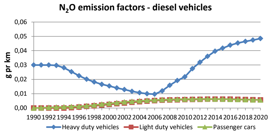
Figure 4.13 Fuel and km related N 2 O emission factors per vehicle type for Danish road transport (1990-2020).
