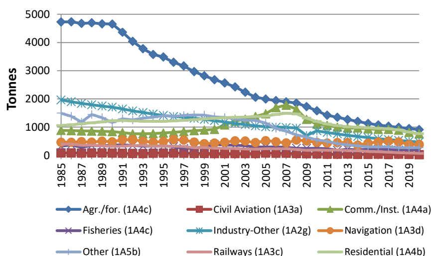
Figure 6.33 NMVOC emissions (tonnes) in NFR sectors for other mobile sources 1985-2020.
