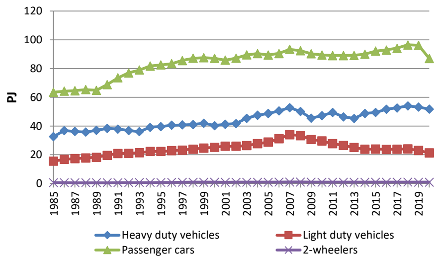
Figure 6.4 Total fuel consumption per vehicle type for road transport 1985-2020.
