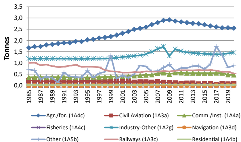
Figure 6.37 NH 3 emissions (tonnes) in NFR sectors for other mobile sources 1985-2020.
