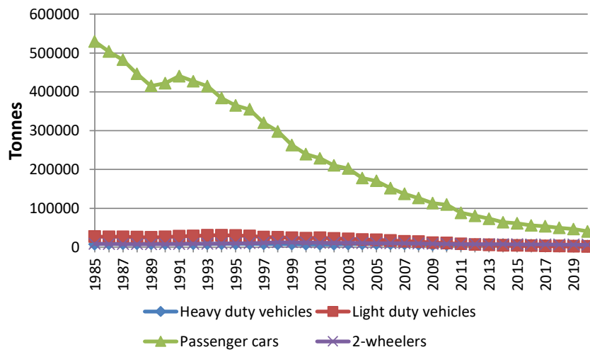
Figure 6.25 CO emissions (tonnes) per vehicle type for road transport 1985-2020.
