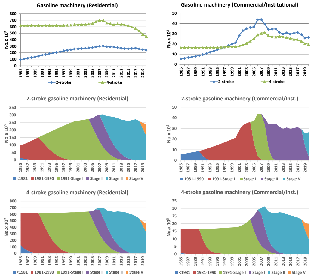
Figure 5.10 Layer distribution for the most important household and gardening machinery types split into residential and commercial/institutional (1985-2020).
