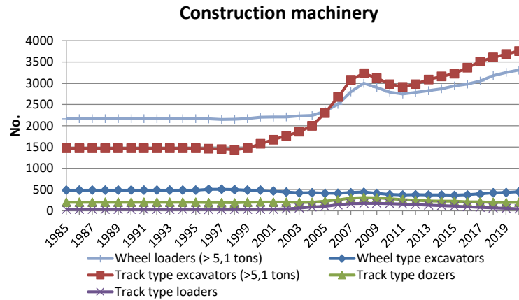
Figure 5.6 1985-2020 stock development for specific types of construction machinery.
