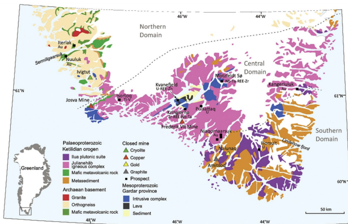
Takussutissiaq A1.1. Major tectonic units of South Greenland with main mineral occurrences and domains. After Steenfelt et al., 2016.
