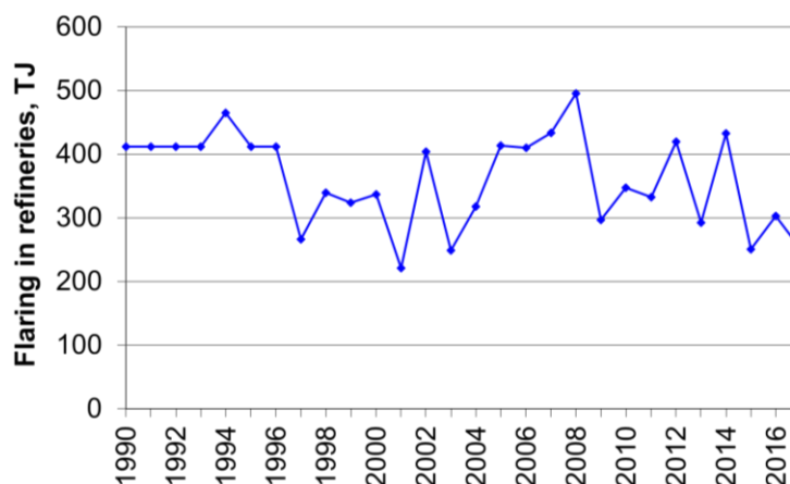
Figure 3.5.14 Flaring rates in refineries.
