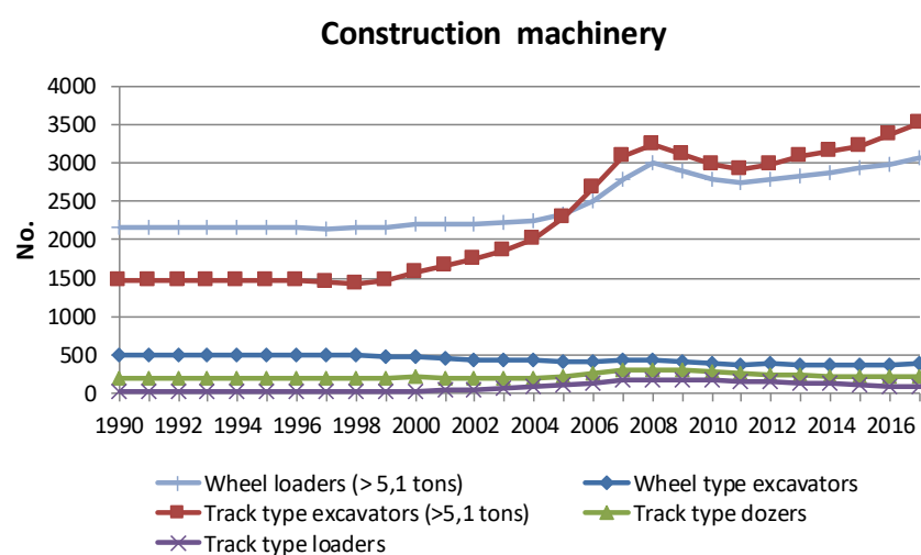
Figure 3.3.35 1990-2017 stock development for specific types of construction machinery.
