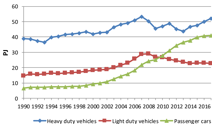
Figure 3.3.6 Diesel fuel consumption per vehicle type for road transport 1990-2017.
