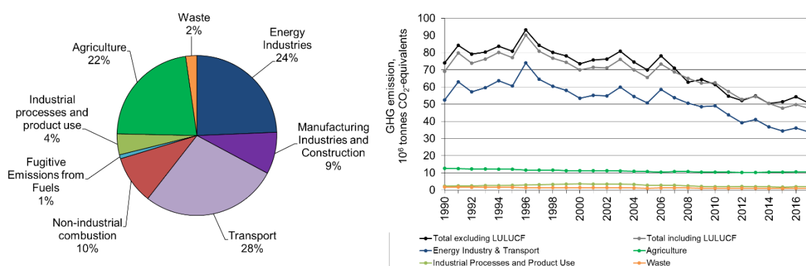
Figure ES.1 Greenhouse gas emissions in CO 2 equivalents distributed on main sectors for 2017 (excluding LULUCF and indirect CO 2 ) and time series for 1990 to 2017.
