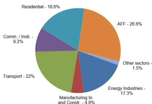
Figure 16.2.4 CO 2 emissions, distribution according to the main sectors for 2017.
