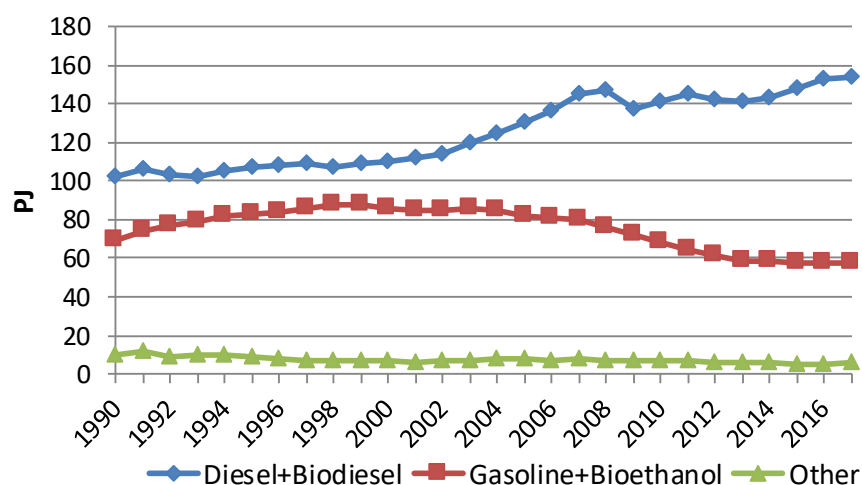
Figure 3.3.1 Fuel consumption per fuel type for domestic transport 1990-2017.
