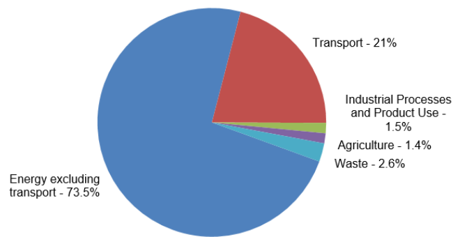
Figure 16.2.2 Greenhouse gas emission in CO 2 equivalents distributed on main sectors for 2017.
