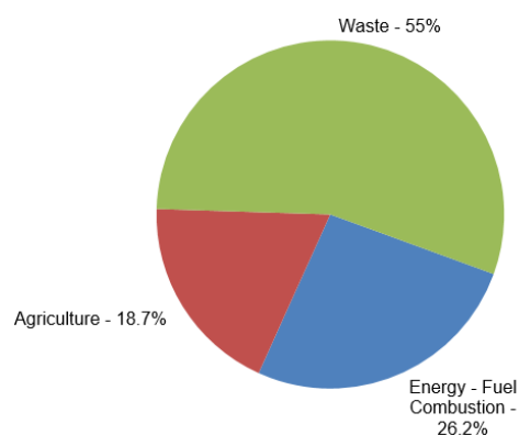
Figure 16.2.6 N 2 O emissions, distribution according to the main sectors in 2017.
