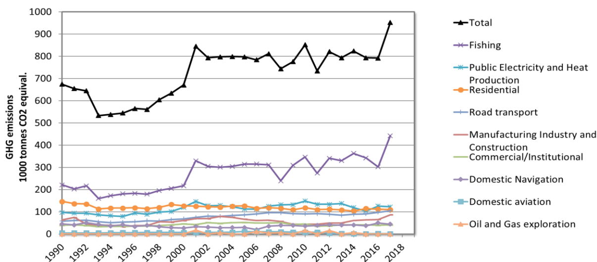
Figure 11 GHG emissions in CO 2 equivalents, categories in the Energy sector, 1990-2017.
