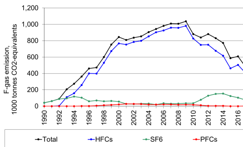
Figure 2.5 F-gas emissions. Time series for 1990 to 2017.
