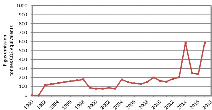
Figure 14 Emission of SF 6 in CO 2 equivalents, time series for Electrical Equipment, 1990-2017.
