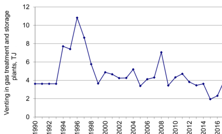
Figure 3.5.13 Venting rates in gas storage facilities.
