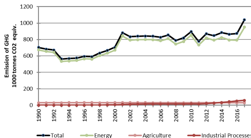
Figure 9 GHG emissions in CO 2 equivalents, main sectors, time series 1990-2017.
