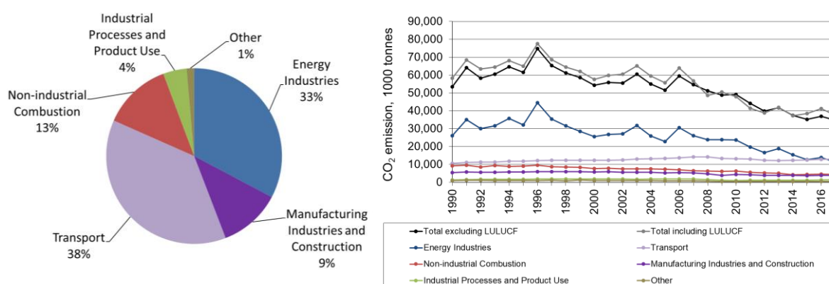
Figure 2.2 CO 2 emissions. Distribution according to the main sectors for 2017 and time series for 1990 to 2017.
