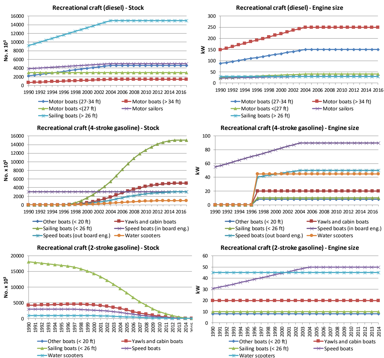
Figure 3.3.40 1990-2017 Stock and engine size development for recreational craft.
