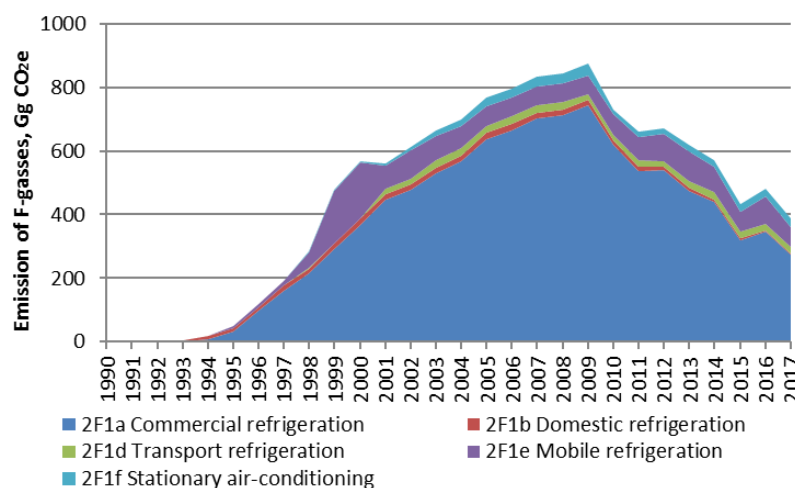
Figure 4.7.3 Emissions from refrigeration and air-conditioning.
