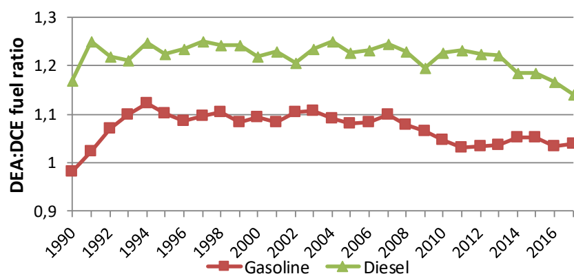
Figure 3.3.26 Gasoline and diesel fuel ratios (fuel and emission adjustment factors) regardless of vehicle category: Fuel sold and used in Denmark vs adjusted bottom-up fuel consumption.
