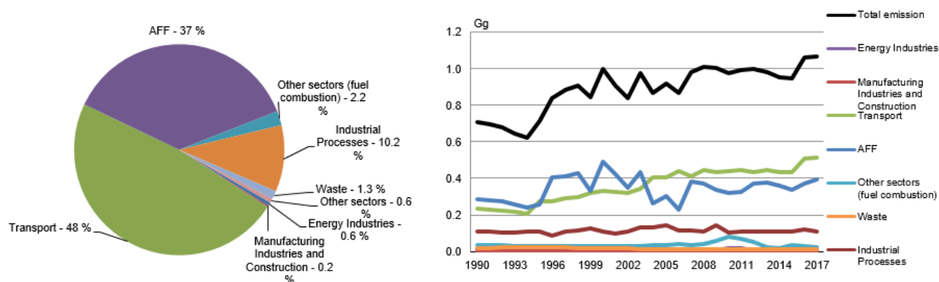
Figure 16.2.12 NMVOC emissions. Distribution according to the main sectors (2017), and time series (1990-2017).
