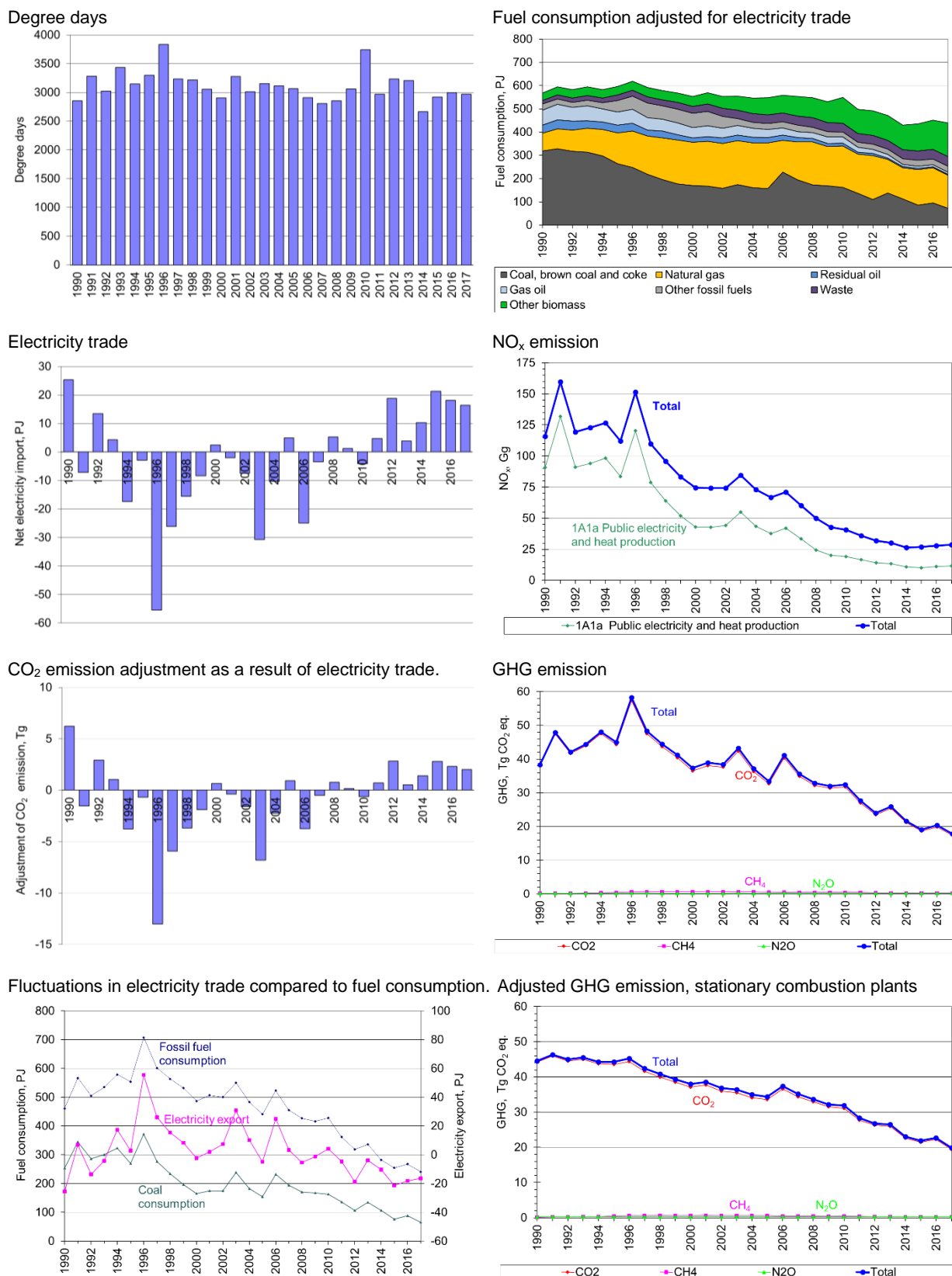
Figure 3.2.4 Comparison of time series fluctuations for net electricity import, fuel consumption, CO 2 emission and NO x emission. Based on DEA (2018a).
