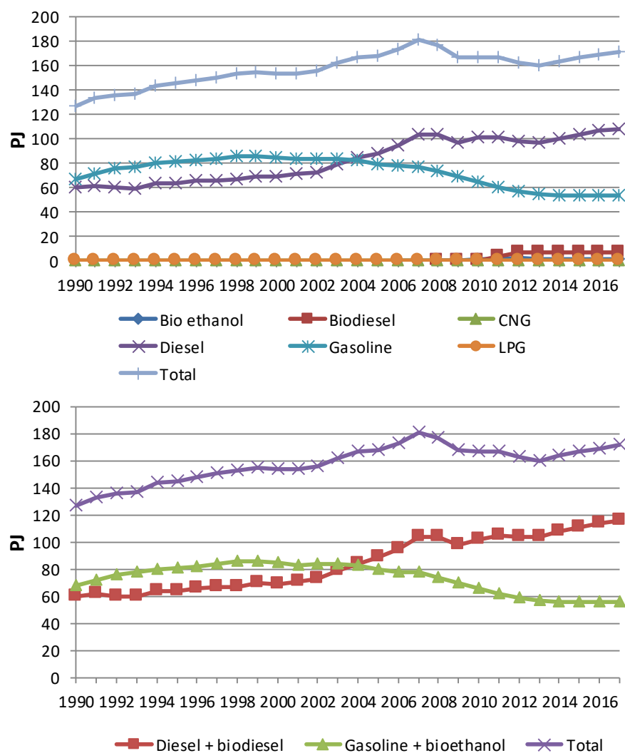
Figure 3.3.3 Fuel consumption per fuel type and as totals for road transport 1990-2017.
