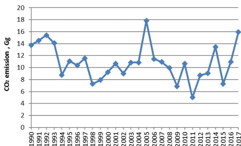
Figure 4.2.6 \text{CO}_2 emissions from other uses of soda ash.
