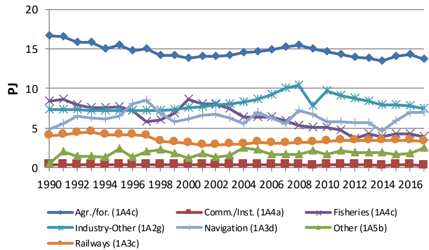
Figure 3.3.9 Diesel fuel consumption in CRF sectors for other mobile sources 1990-2017.
