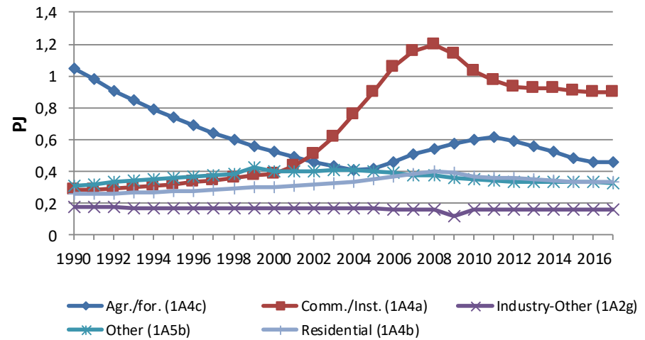
Figure 3.3.10 Gasoline fuel consumption in CRF sectors for other mobile source 1990-2017.
