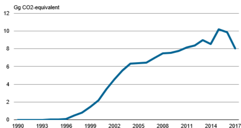
Figure 16.4.4 Emission of HFCs (from refrigeration).
