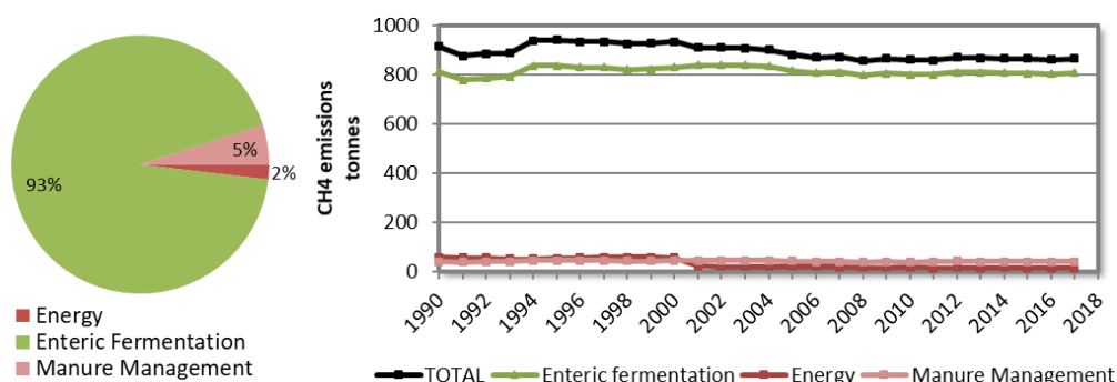
Figure 7 CH 4 emissions in tonnes distributed on sectors and time series for 1990-2017.
