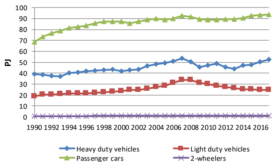
Figure 3.3.4 Total fuel consumption per vehicle type for road transport 1990-2017.
