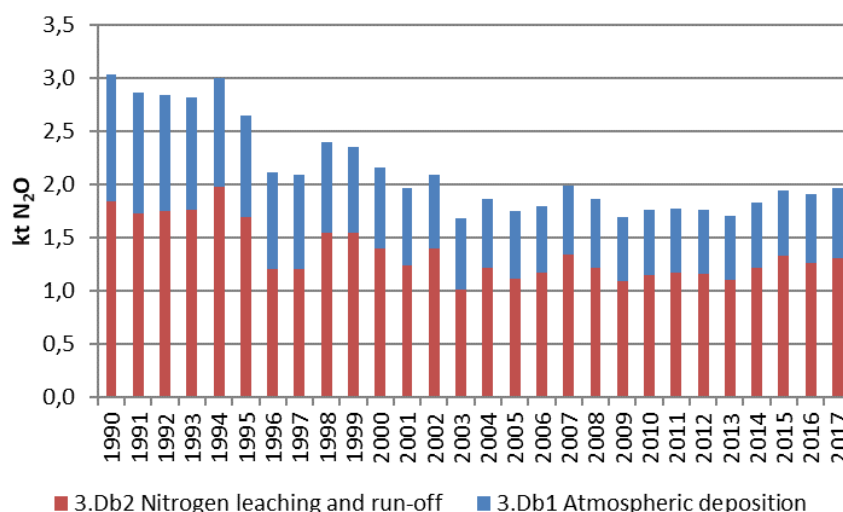
Figure 5.12 N 2 O emissions from agricultural soils – indirect emissions 1990 – 2017.
