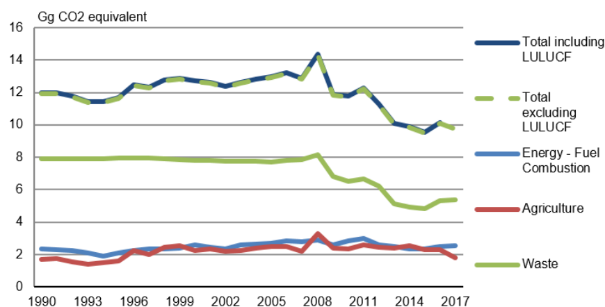
Figure 16.2.5 N 2 O emissions, time-series for 1990-2017.
