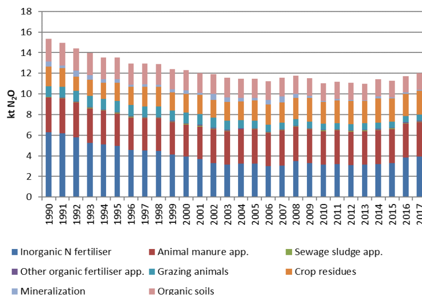
Figure 5.10 N 2 O emissions from agricultural soils – direct emissions 1990 - 2017.
