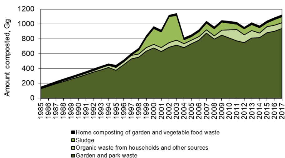
Figure 7.3.2 Trends in the national amount of composted waste.
