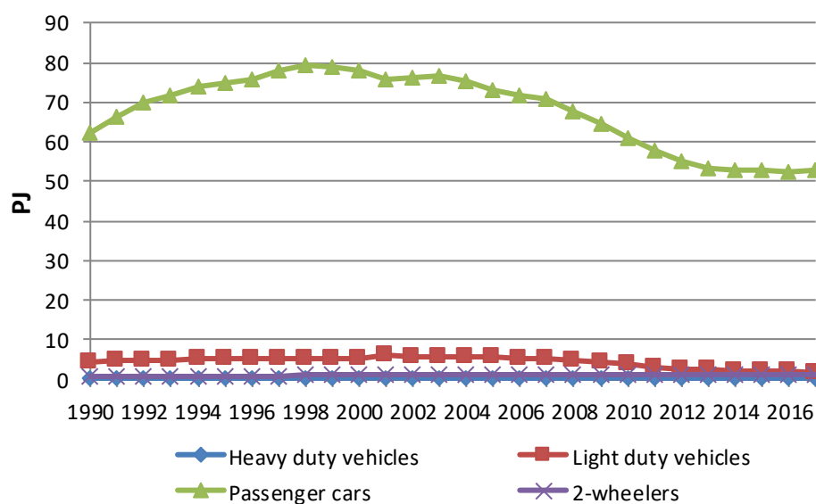
Figure 3.3.5 Gasoline fuel consumption per vehicle type for road transport 1990-2017.
