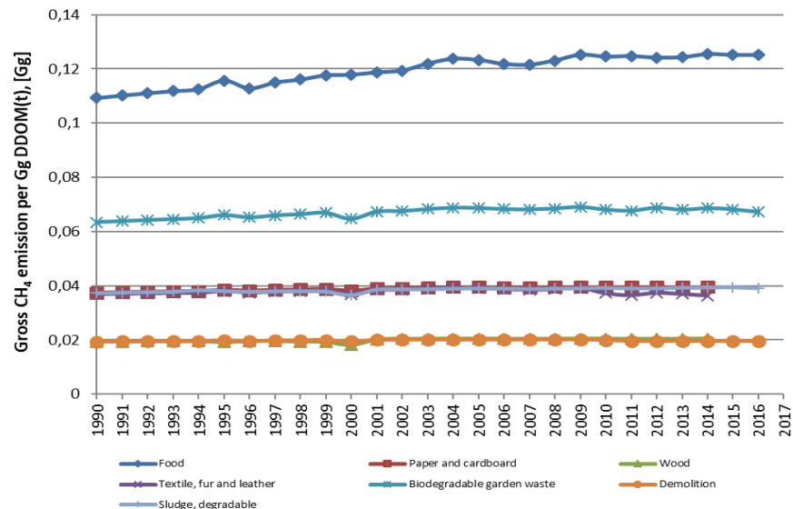
Figure 7.2.2 Annual gross implied emission factors for each waste type.
