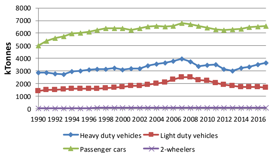
Figure 3.3.14 CO 2 emissions (k-tonnes) per vehicle type for road transport 1990-2017.
