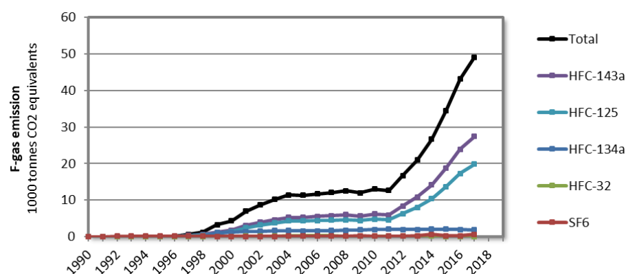
Figure 13 Emissions of f-gases, in CO 2 equivalents, Industrial processes and Product Use, 1990-2017.
