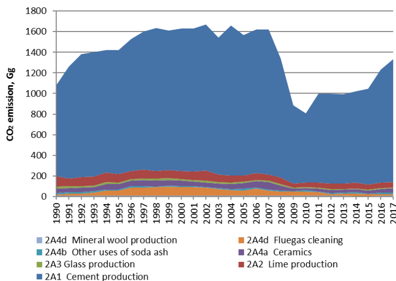
Figure 4.2.1 Emission of CO 2 from the individual source categories compiling 2A Mineral Industry , Gg.
