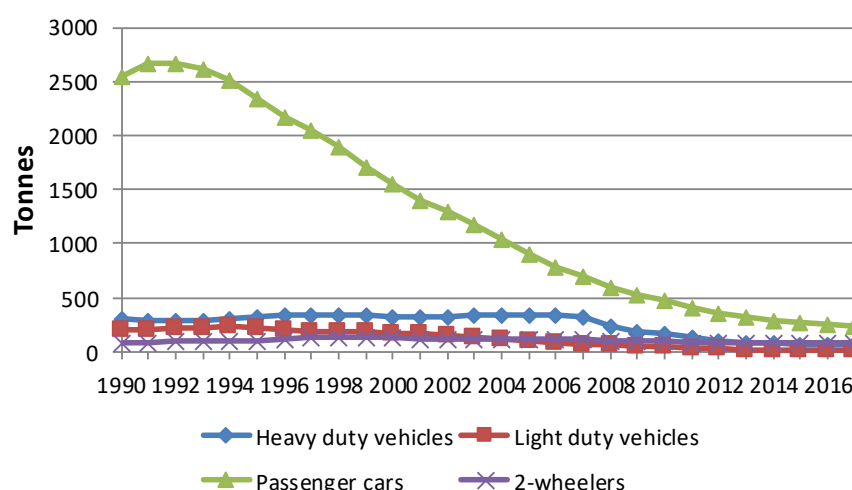
Figure 3.3.15 CH 4 emissions (tonnes) pr. vehicle type for road transport 1990-2017.
