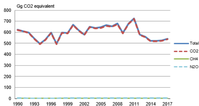
Figure 16.3.5 GHG emission time-series for the Energy Sector.
