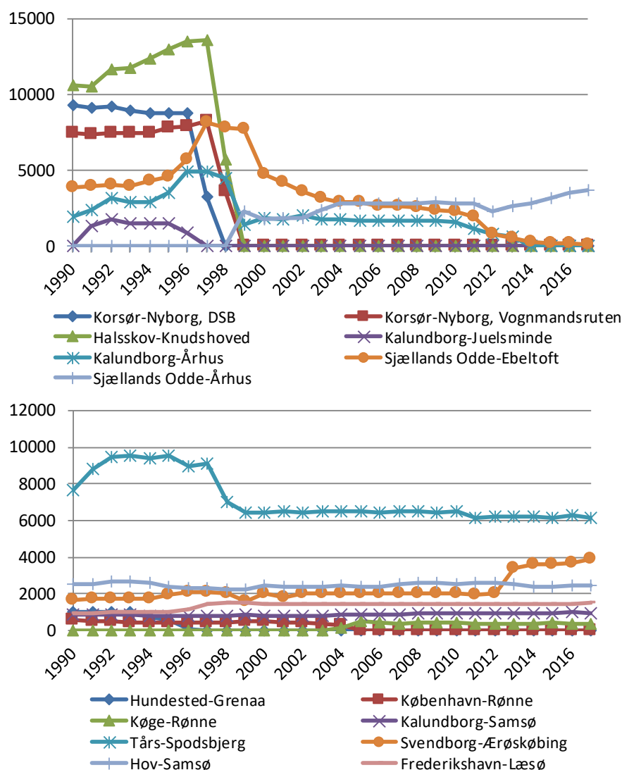
Figure 3.3.42 No. of round trips for the most important ferry routes in Denmark 1990-2017.
