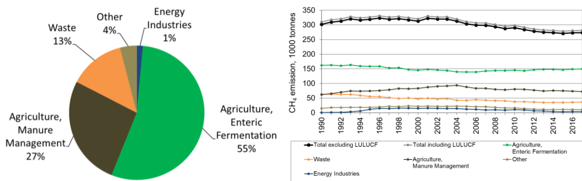
Figure 2.3 CH 4 emissions. Distribution according to the main sectors for 2017 and time series for 1990 to 2017.
