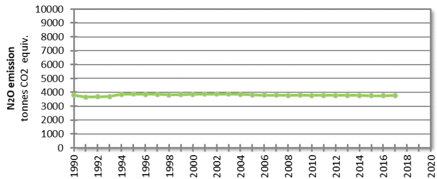
Figure 19 N 2 O emissions (tonnes CO 2 equiv.) from Agricultural Soils, time series 1990-2017.
