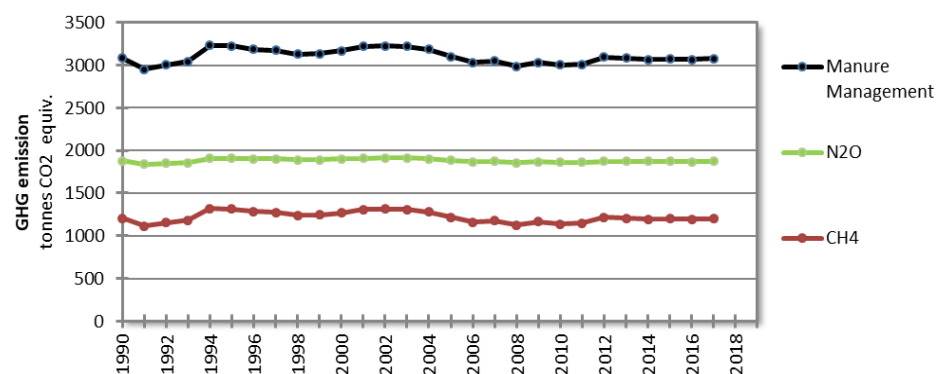
Figure 18 N 2 O and CH 4 emission in CO 2 equivalents from Manure management, time series 1990-2017.
