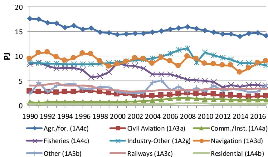
Figure 3.3.8 Total fuel consumption in CRF sectors for other mobile sources 1990-2017.
