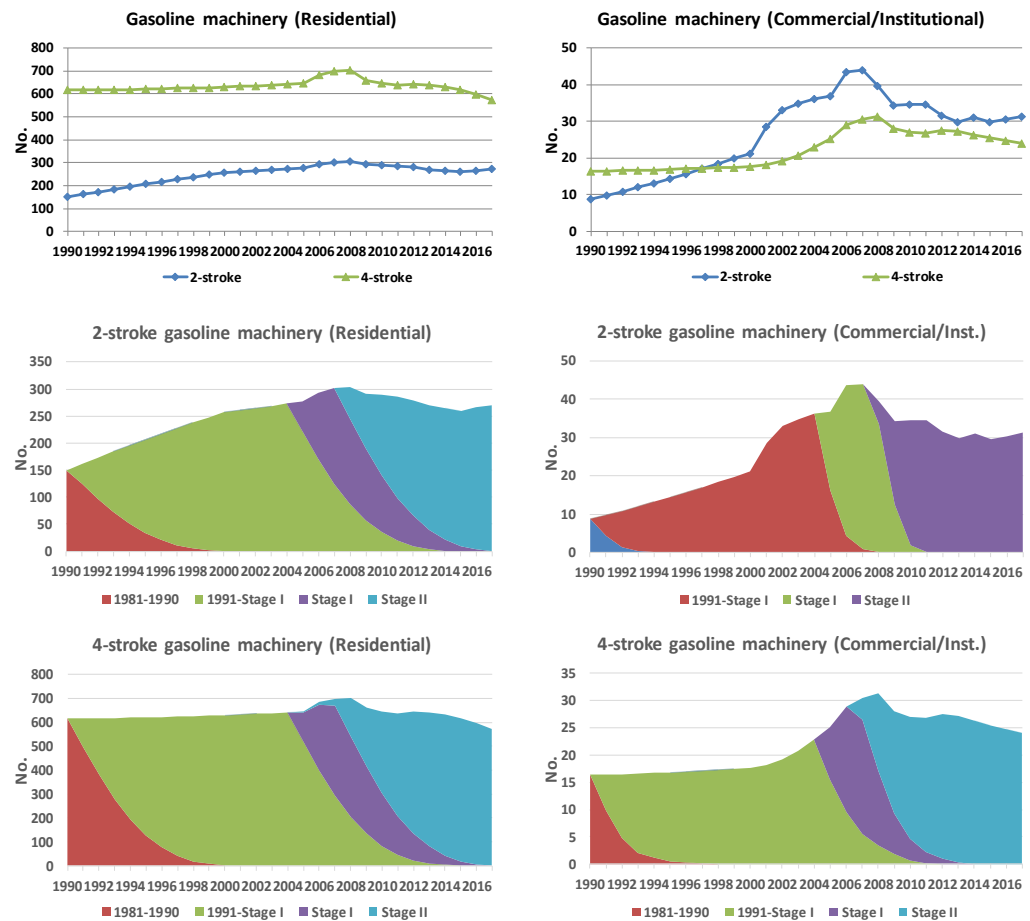
Figure 3.3.39 Layer distribution for the most important household and gardening machinery types split into residential and commercial/institutional (1990-2017).
