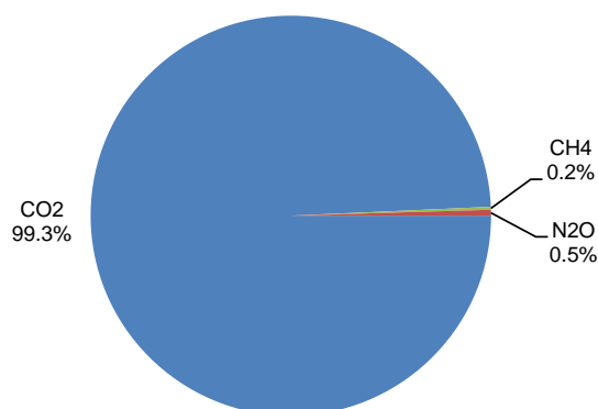
Figure 16.3.4 GHG emissions (CO 2 equivalent) from stationary combustion plants 2017.
