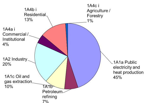
Fuel consumption, fossil fuels
