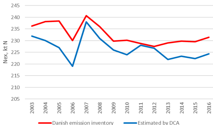
Figure 5.16 Comparison of Nex estimated by DCE and DCA
