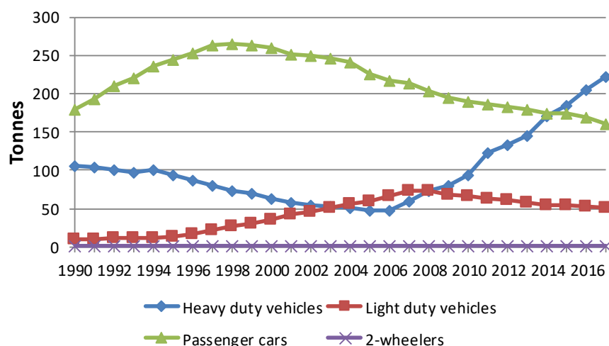
Figure 3.3.16 N 2 O emissions (tonnes) per vehicle type for road transport 1990-2017.
