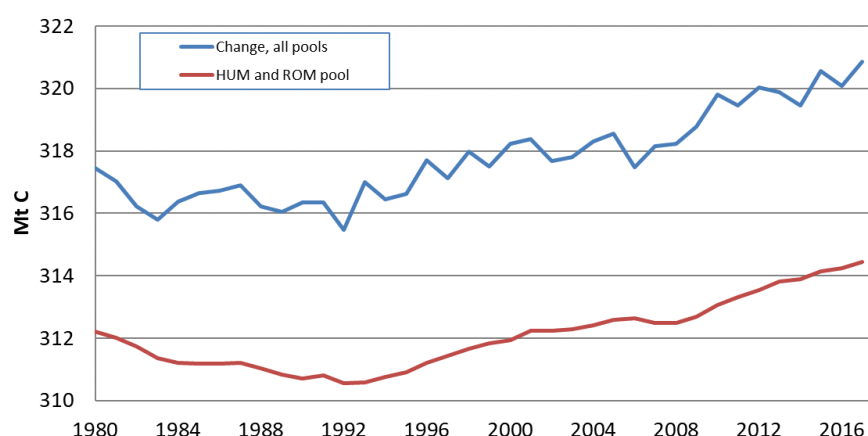
Figure 6.6 The development in the C-stock in agricultural soils, 1980-2017, Mt C (million tonne C).
