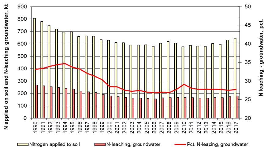
Figure 5.11 Nitrogen applied to agricultural soils and N-leaching, groundwater 1990-2017.
