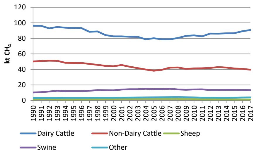
Figure 5.4 Emission of CH 4 from enteric fermentation, 1990-2017. For all numbers see Annex 3D Table 3D-13.
