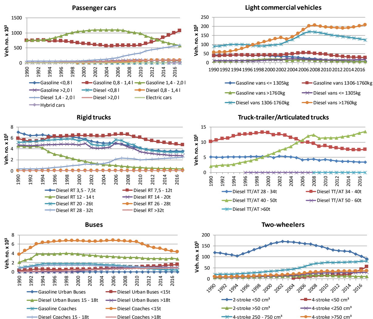
Figure 3.3.23 Number of vehicles in sub-classes in 1990-2017.
