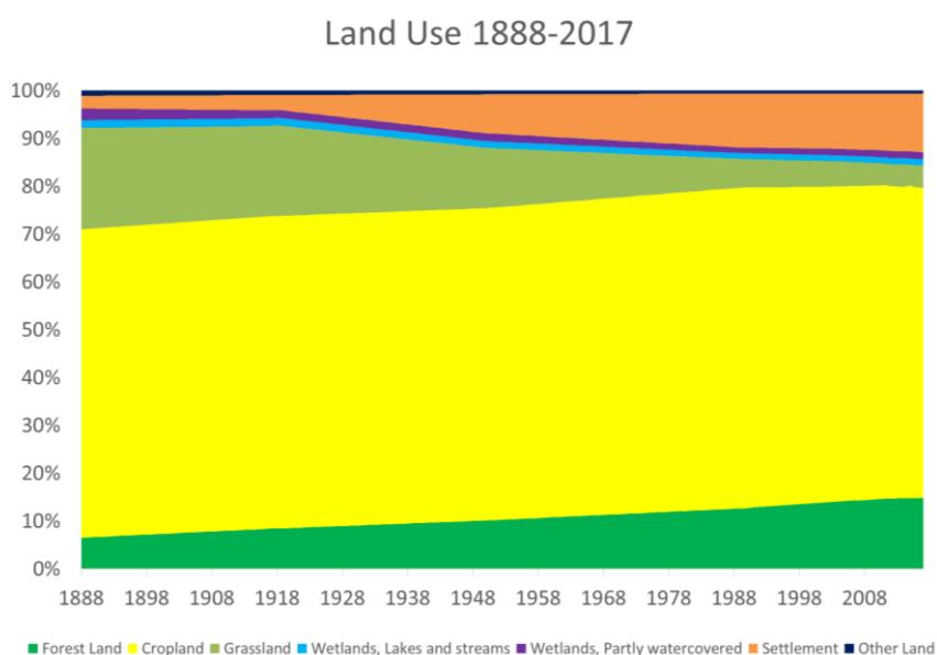
Figure 3E.5 Land Use Change 1888-2017.
