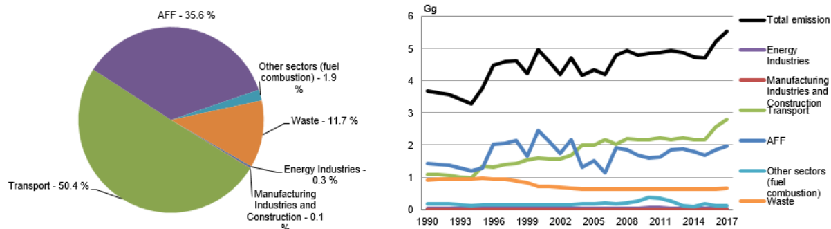
Figure 16.2.11 CO emissions. Distribution according to the main sectors (2017), and time series (1990-2017).
