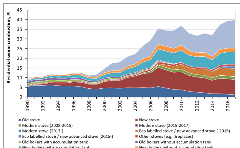
Figure 3.2.37 Technology specific wood consumption in residential plants.
