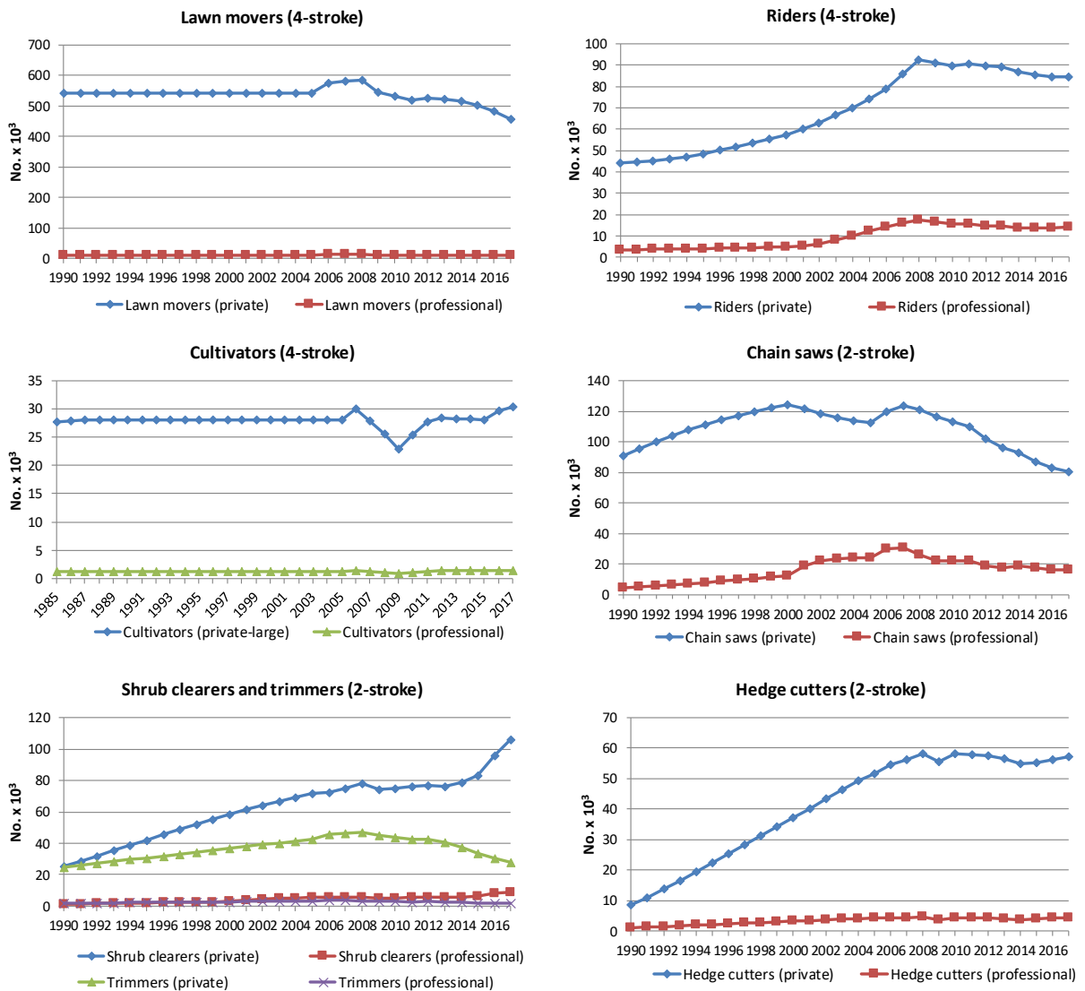
Figure 3.3.38 Stock development 1990-2017 for the most important household and gardening machinery types.
