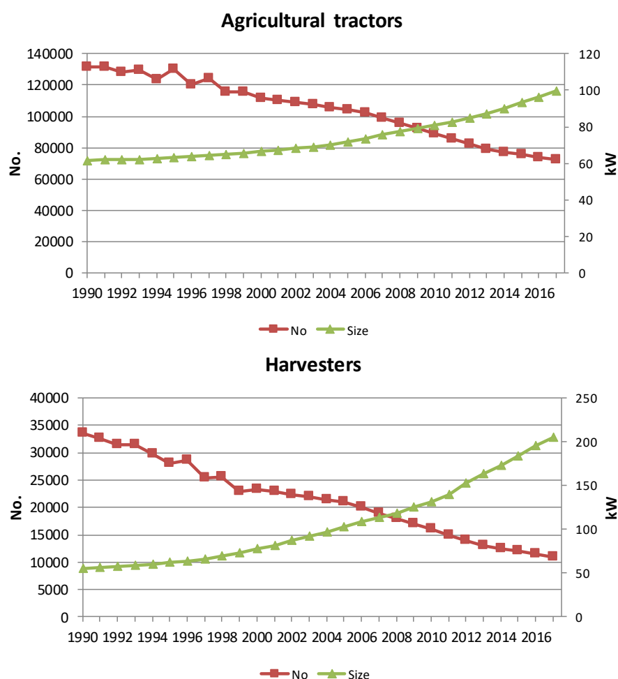
Figure 3.3.34 Total numbers and average engine size for agricultural tractors and harvesters (1990 to 2017).
