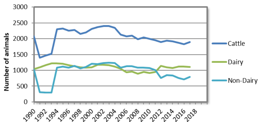
Figure 15 Number of cattle (dairy and non-dairy), time series for 1990-2017.
