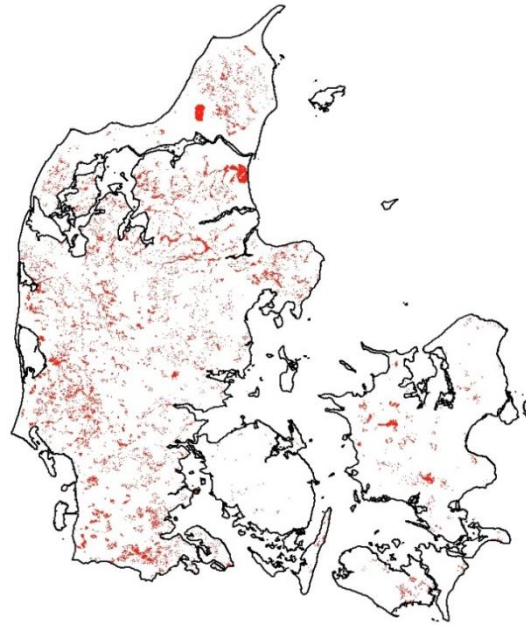
Figure 6.9 The new organic soil map for Denmark for year 2010, > 12 % OC (Greve et al. 2014).
