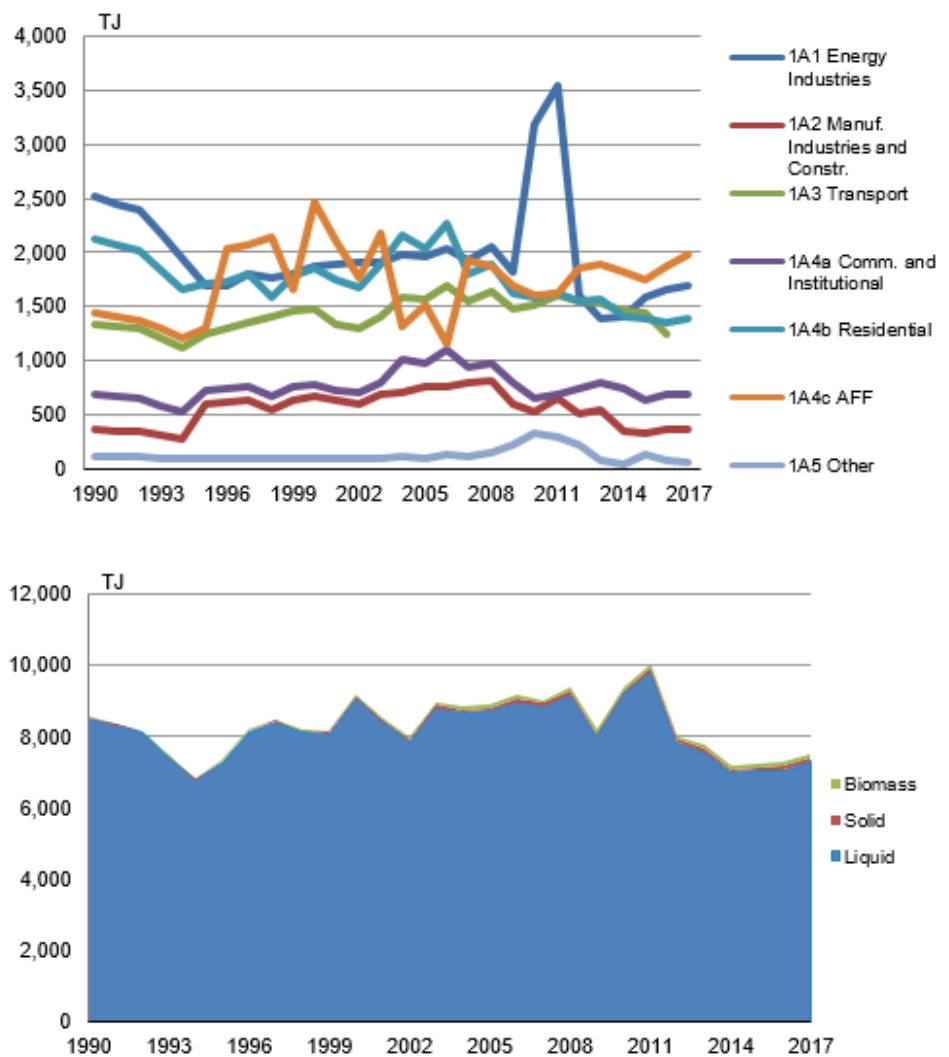
Figure 16.3.3 Fuel consumption time-series 1990-2017.
