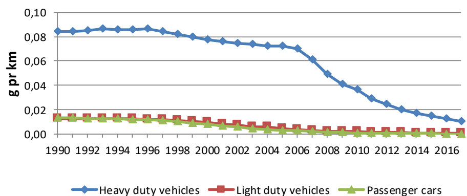
Figure 3.3.28 Fuel and km related CH 4 emission factors per vehicle type for Danish road transport (1990-2017).
