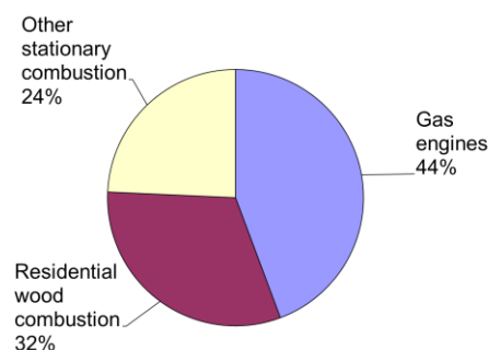
Figure 3.2.12 CH 4 emission share for gas engines and residential wood combustion, 2017.
