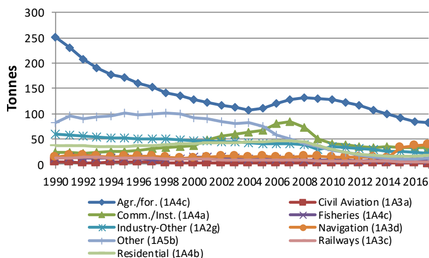
Figure 3.3.19 CH 4 emissions (tonnes) in CRF sectors for other mobile sources 1990-2017.
