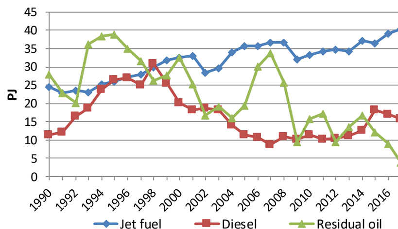
Figure 3.3.13 Bunker fuel consumption 1990-2017.
