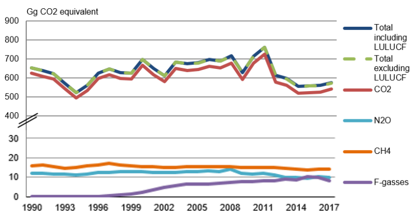
Figure 16.2.1 Greenhouse gas emission in CO 2 equivalents, time-series 1990-2017.
