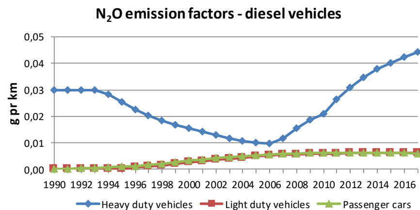
Figure 3.3.29 Fuel and km related N 2 O emission factors per vehicle type for Danish road transport (1990-2017).
