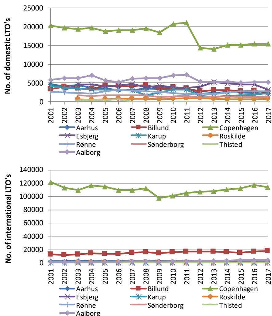
Figure 3.3.31 No. of LTO's for the most important airports in Denmark 2001-2017.
