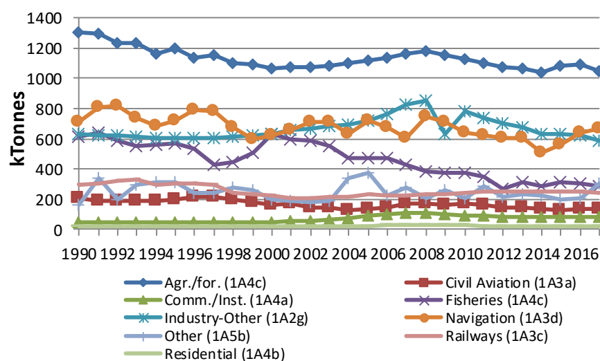
Figure 3.3.18 CO 2 emissions (ktonnes) in CRF sectors for other mobile sources 1990-2017.
