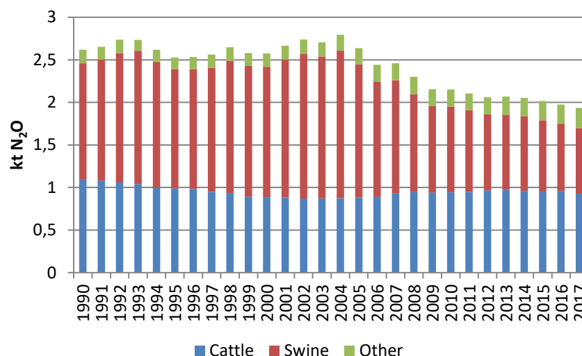
Figure 5.6 N 2 O direct emission from manure management, 1990 - 2017.
