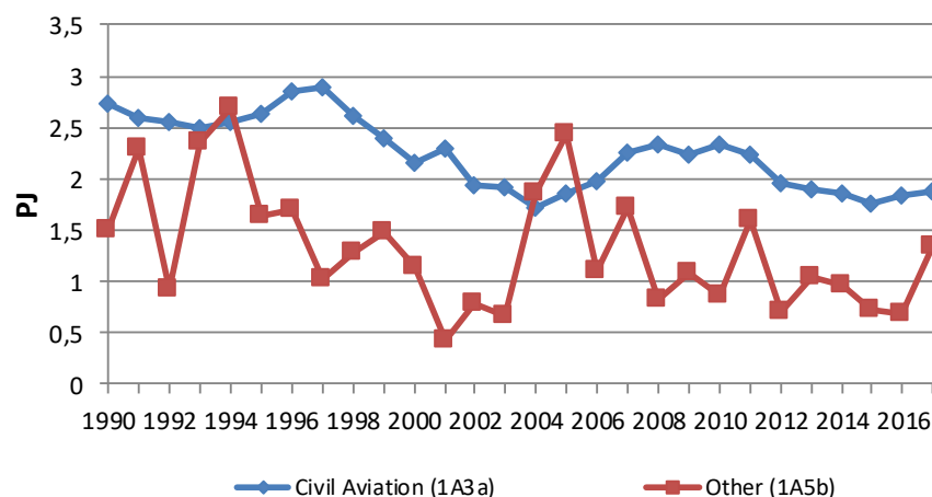
Figure 3.3.12 Jet fuel consumption in CRF sectors for other mobile sources 1990-2017.
