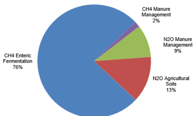
Figure 16.5.1 Emission of greenhouse gases from agriculture in 2017.
