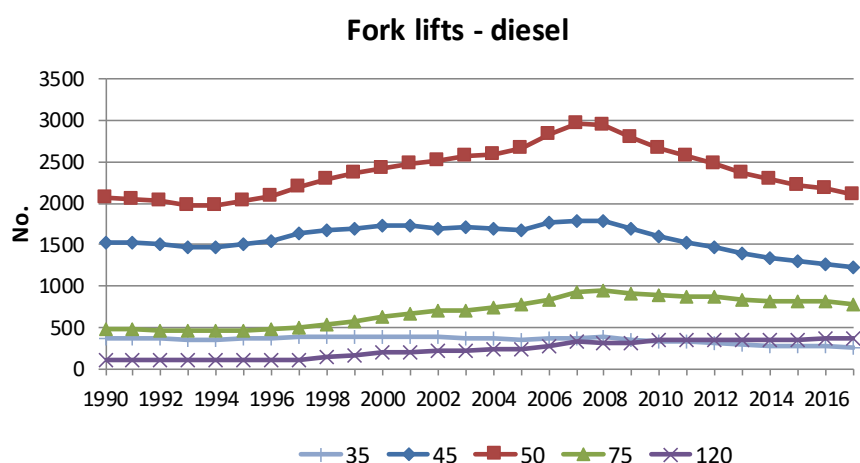
Figure 3.3.36 Total numbers of diesel fork lifts in kW classes from 1990 to 2017.
