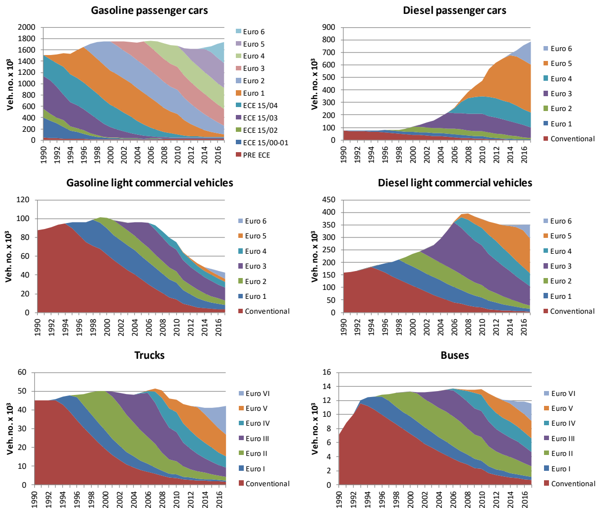
Figure 3.3.24 Layer distribution of vehicle numbers per vehicle type in 1990-2017.
