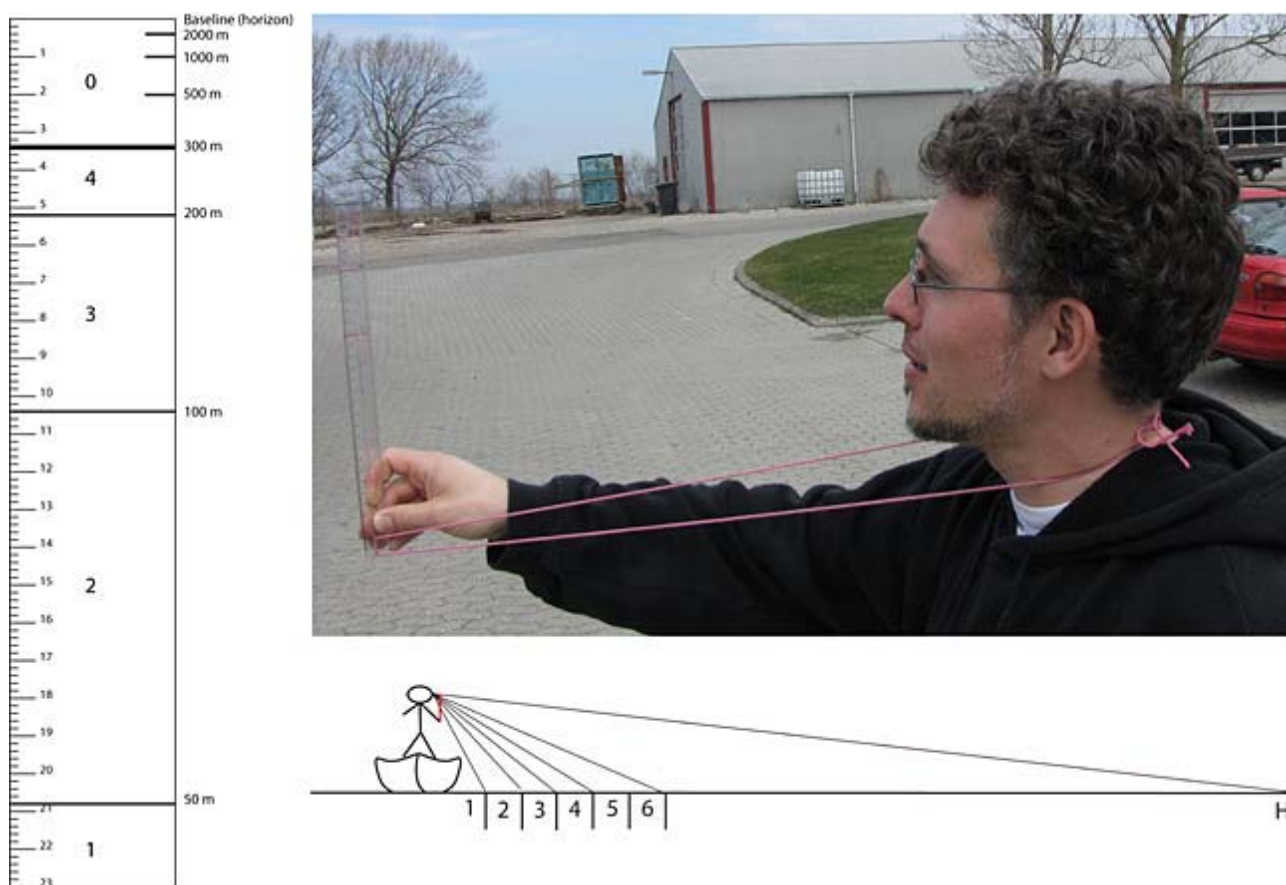
Figure 7. Left: Example of a range stick for transect type A (300 m strip width) with the top of the ruler as baseline. The large figures on the ruler are the distance codes used for the bands of the transect strip. A few additional marks for assessing long distances to marine mammals are included. Upper, right: Illustration of how the range stick may be held at a consistent distance from the eye by means of a string around the neck. Remember to adjust the length of the string according to the thickness of your clothes. Lower, right: Principle sketch of how the delimitation of the distance bands parallel to the track line of the ship are assessed by means of the range stick.
